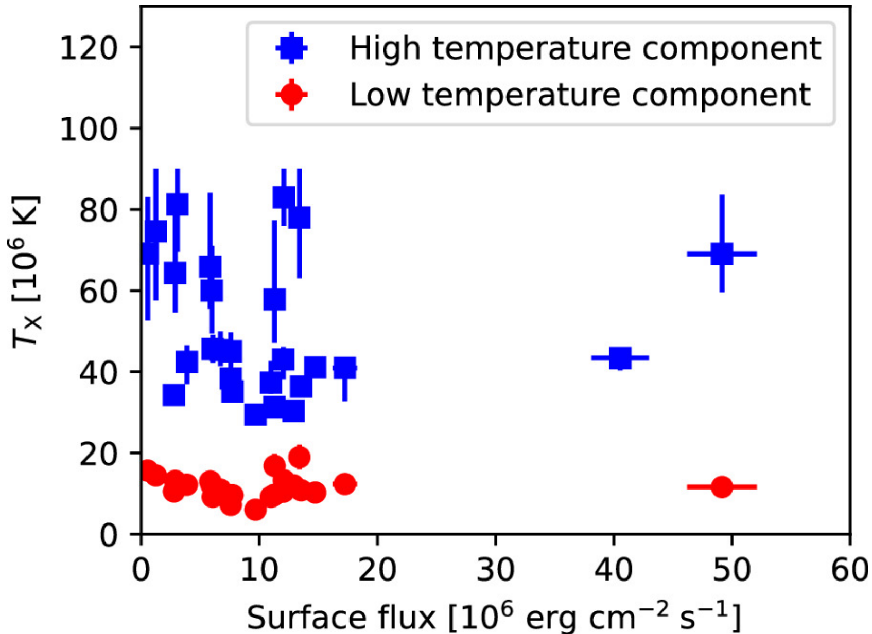
Figure 10. from Norbert S. Schulz et al 2024 Astrophys. J. 970 doi:10.3847/1538-4357/ad47c2 https://dx.doi.org/10.3847/1538-4357/ad47c2 © 2024. The Author(s). Published by the American Astronomical Society.
