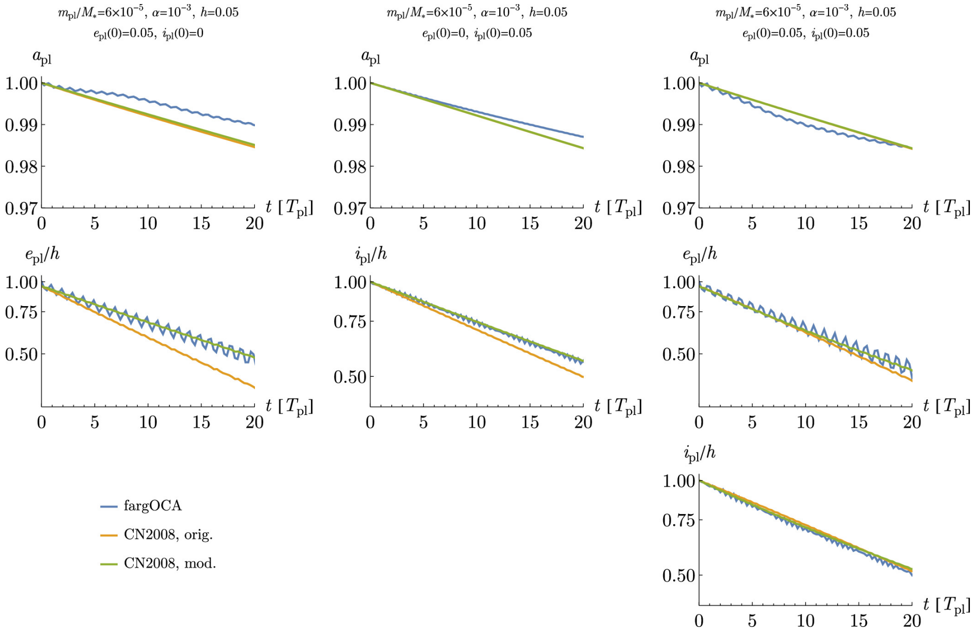
Figure 7. from Gabriele Pichierri et al 2024 Astrophys. J. 967 doi:10.3847/1538-4357/ad3dff https://dx.doi.org/10.3847/1538-4357/ad3dff
