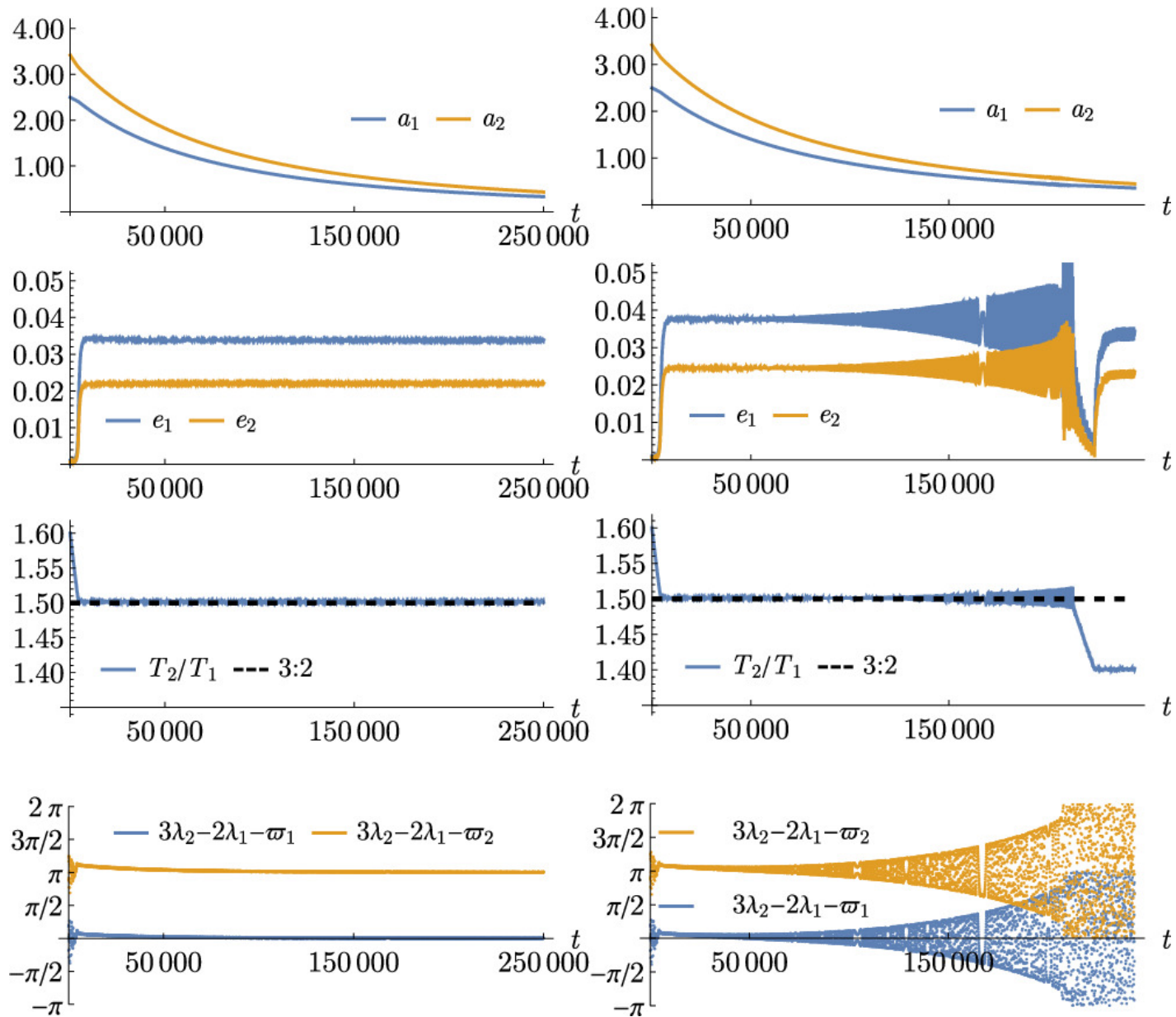
Figure 5. from Gabriele Pichierri et al 2024 Astrophys. J. 967 doi:10.3847/1538-4357/ad3dff https://dx.doi.org/10.3847/1538-4357/ad3dff © 2024. The Author(s). Published by the American Astronomical Society.
