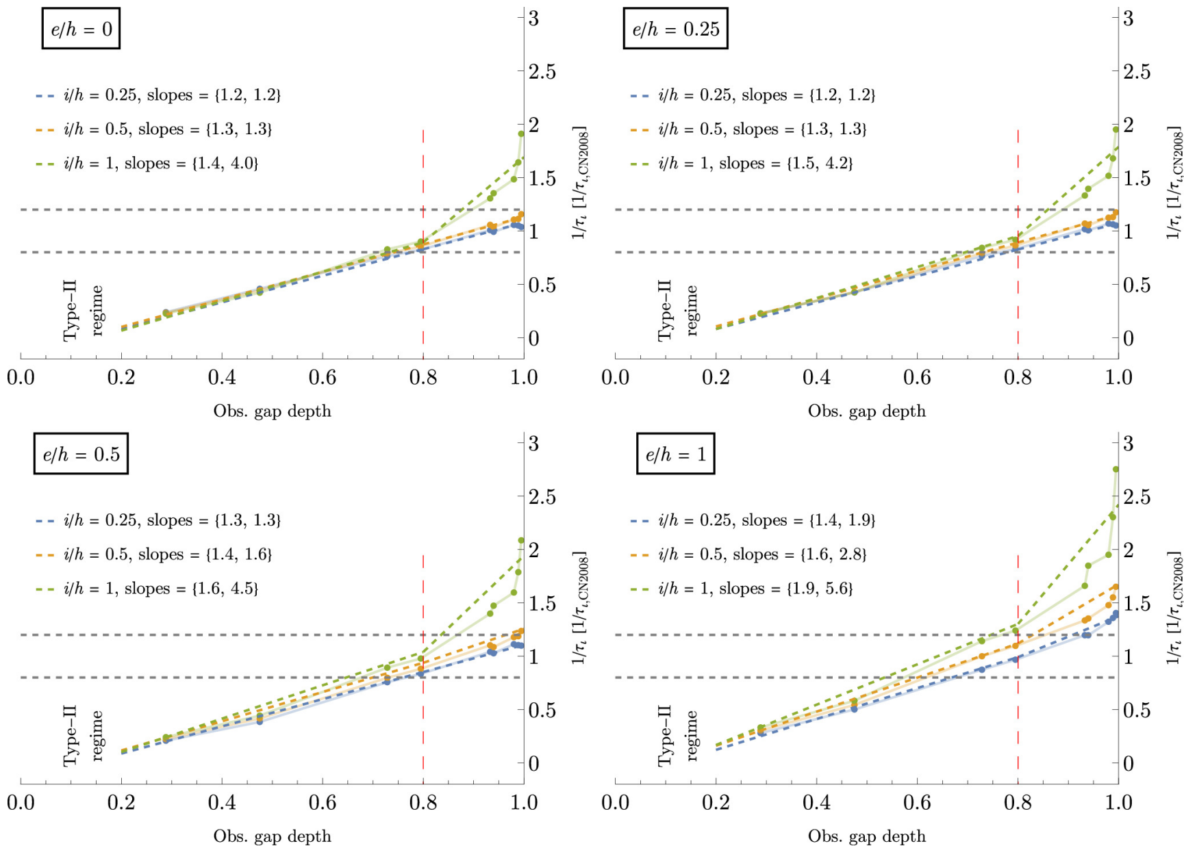
Figure 4. from Gabriele Pichierri et al 2024 Astrophys. J. 967 doi:10.3847/1538-4357/ad3dff https://dx.doi.org/10.3847/1538-4357/ad3dff © 2024. The Author(s). Published by the American Astronomical Society.
