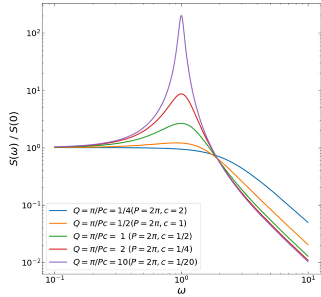
Figure 1. from Fei-Fan Song and Jirong Mao 2024 Astrophys. J. 966 doi:10.3847/1538-4357/ad390a https://dx.doi.org/10.3847/1538-4357/ad390a © 2024. The Author(s). Published by the American Astronomical Society.
