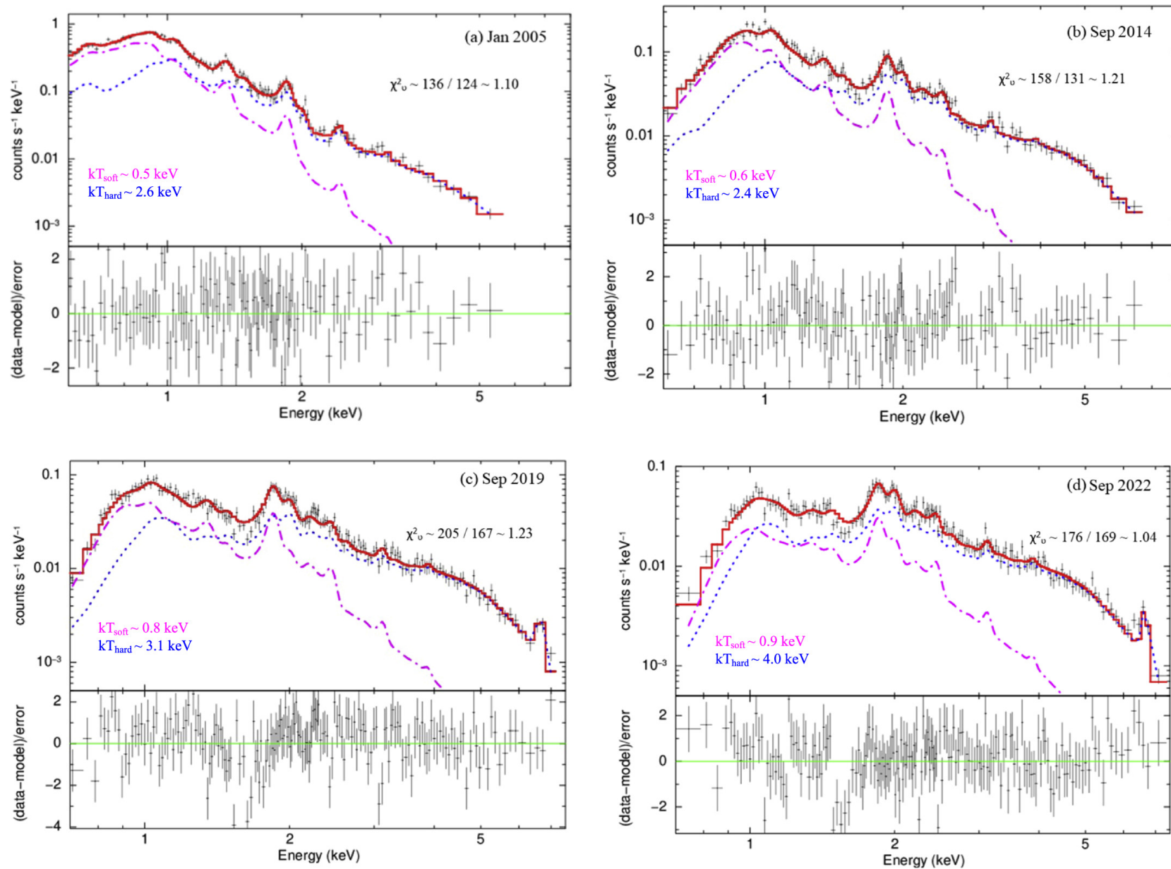
Figure 1. from Aravind P. Ravi et al 2024 Astrophys. J. 966 doi:10.3847/1538-4357/ad3800 https://dx.doi.org/10.3847/1538-4357/ad3800 © 2024. The Author(s). Published by the American Astronomical Society.
