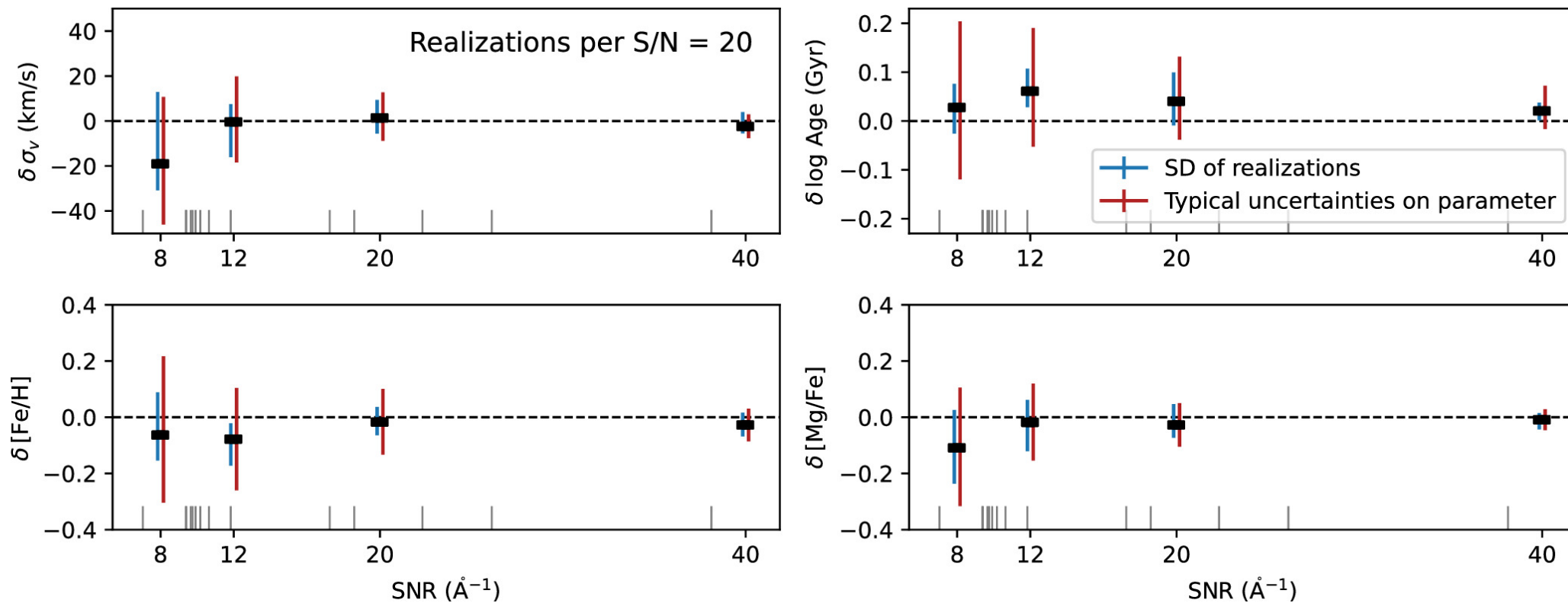
Figure 9. from Aliza G. Beverage et al 2024 Astrophys. J. 966 doi:10.3847/1538-4357/ad372d https://dx.doi.org/10.3847/1538-4357/ad372d © 2024. The Author(s). Published by the American Astronomical Society.
