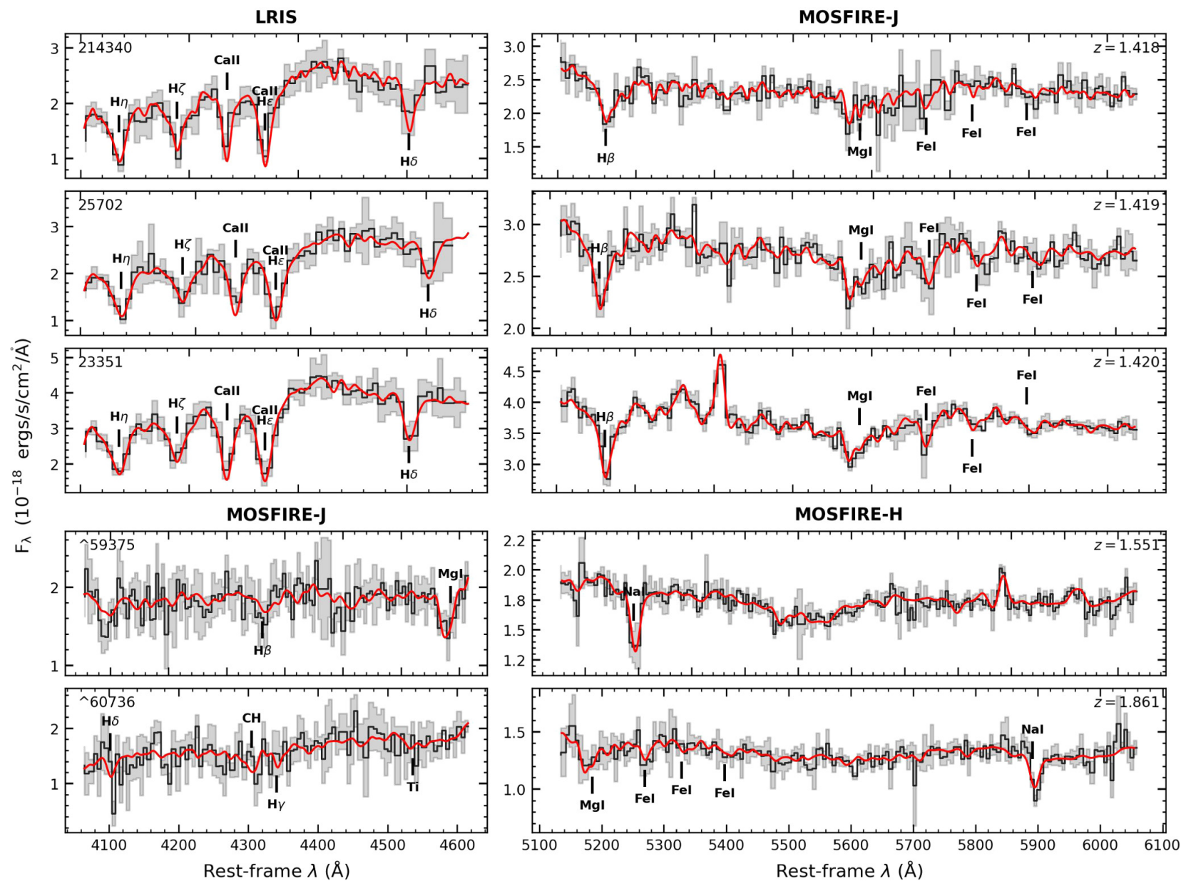
Figure 6. from Aliza G. Beverage et al 2024 Astrophys. J. 966 doi:10.3847/1538-4357/ad372d https://dx.doi.org/10.3847/1538-4357/ad372d © 2024. The Author(s). Published by the American Astronomical Society.
