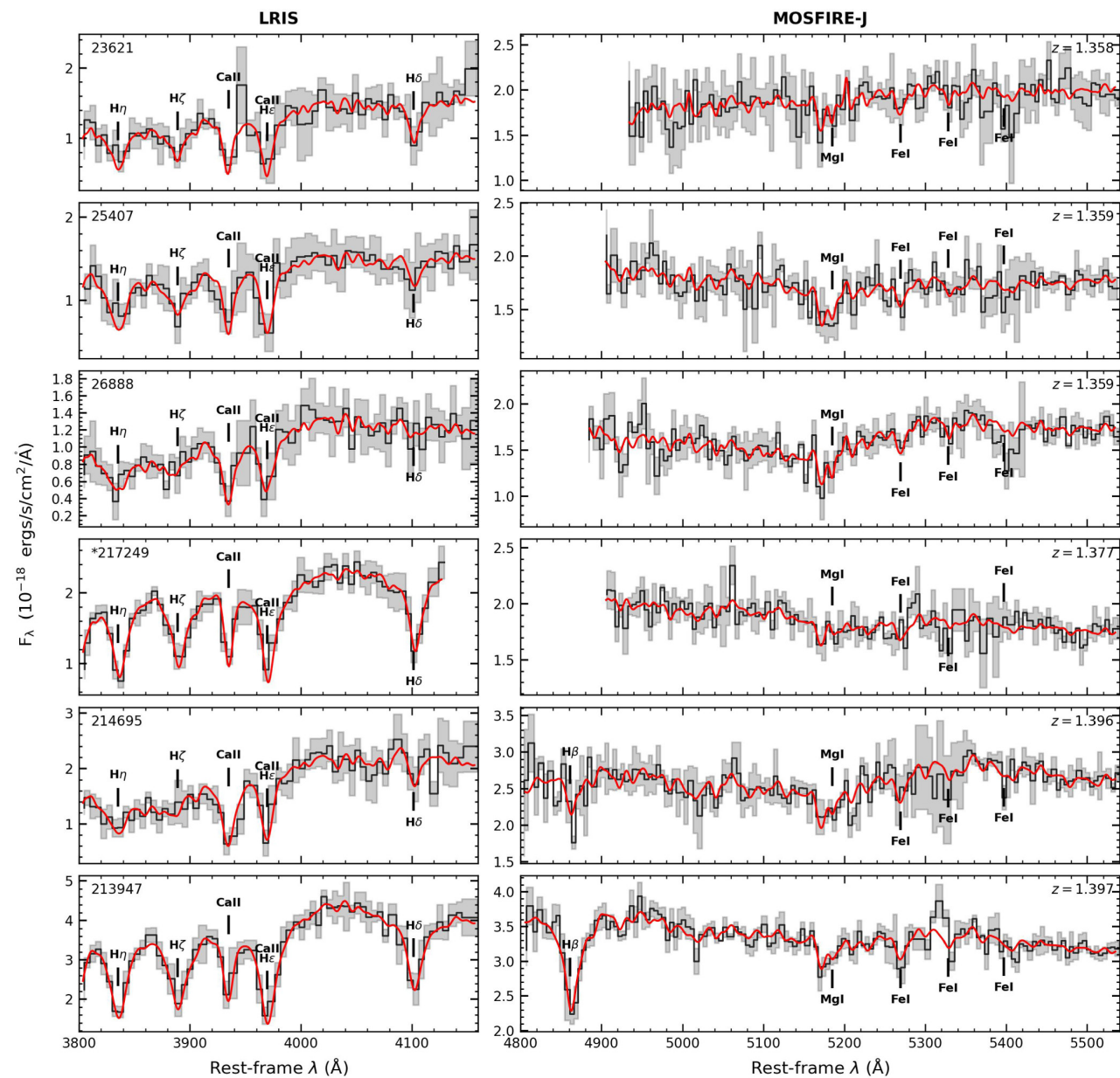
Figure 6. from Aliza G. Beverage et al 2024 Astrophys. J. 966 doi:10.3847/1538-4357/ad372d https://dx.doi.org/10.3847/1538-4357/ad372d © 2024. The Author(s). Published by the American Astronomical Society.
