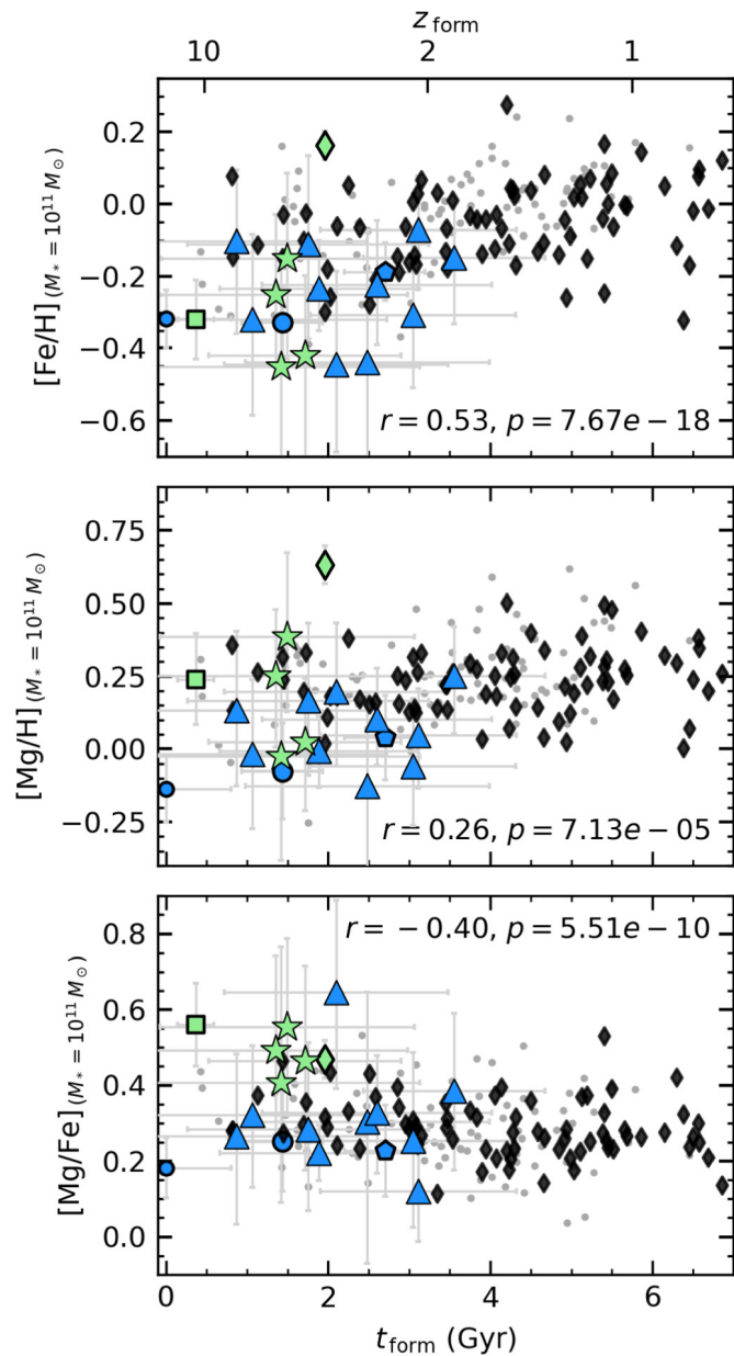
Figure 5. from Aliza G. Beverage et al 2024 Astrophys. J. 966 doi:10.3847/1538-4357/ad372d https://dx.doi.org/10.3847/1538-4357/ad372d © 2024. The Author(s). Published by the American Astronomical Society.
