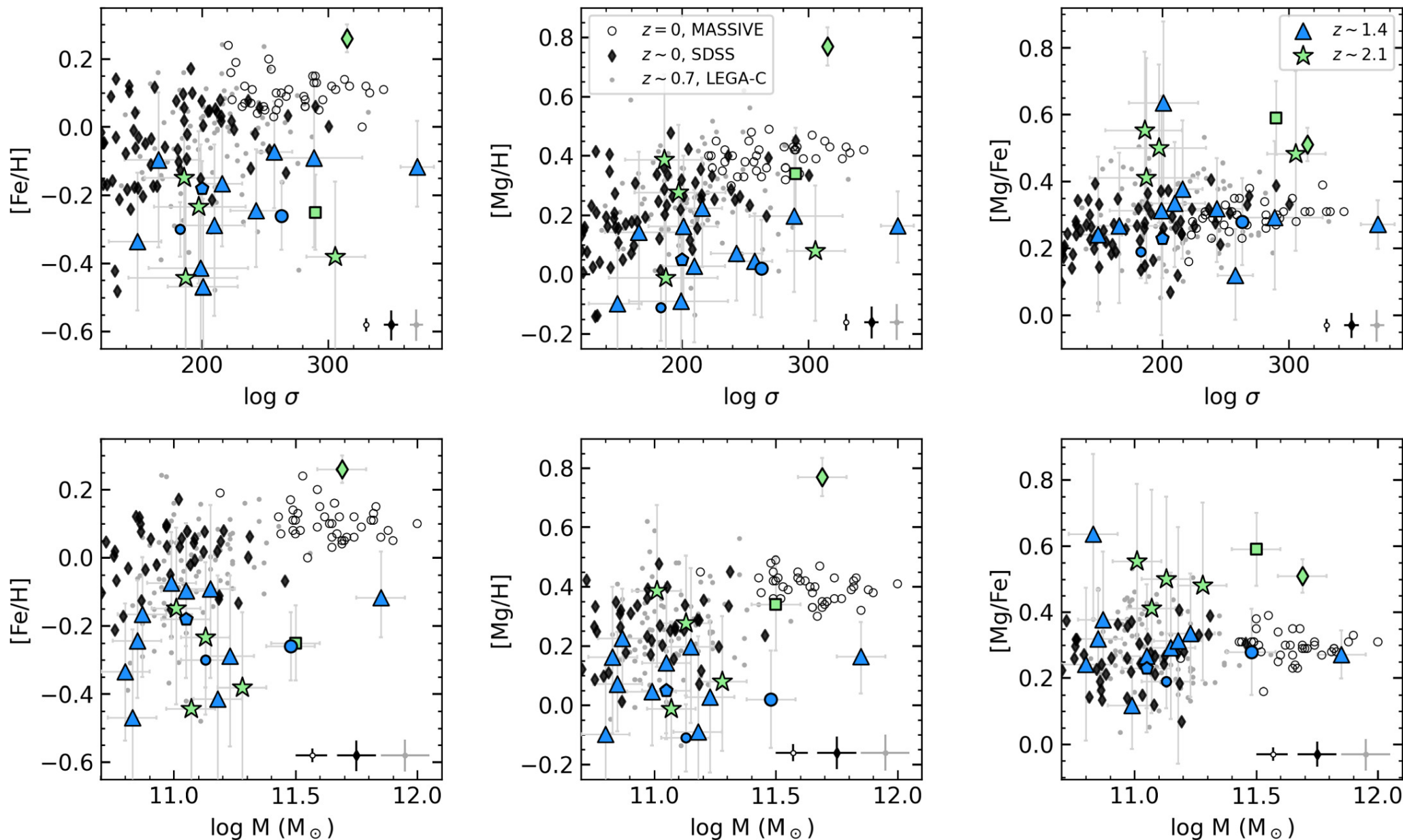
Figure 4. from Aliza G. Beverage et al 2024 Astrophys. J. 966 doi:10.3847/1538-4357/ad372d https://dx.doi.org/10.3847/1538-4357/ad372d © 2024. The Author(s). Published by the American Astronomical Society.
