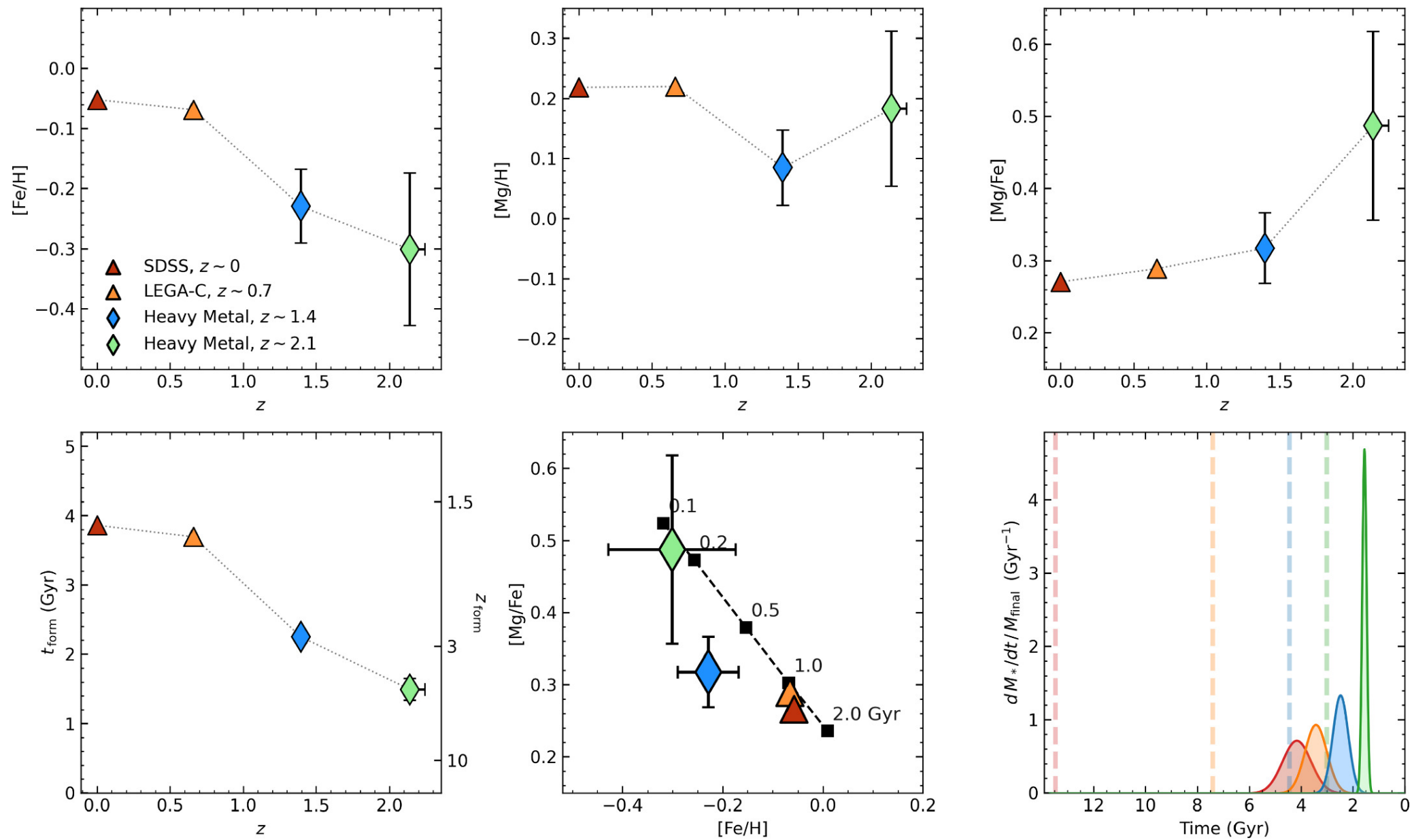
Figure 3. from Aliza G. Beverage et al 2024 Astrophys. J. 966 doi:10.3847/1538-4357/ad372d https://dx.doi.org/10.3847/1538-4357/ad372d © 2024. The Author(s). Published by the American Astronomical Society.
