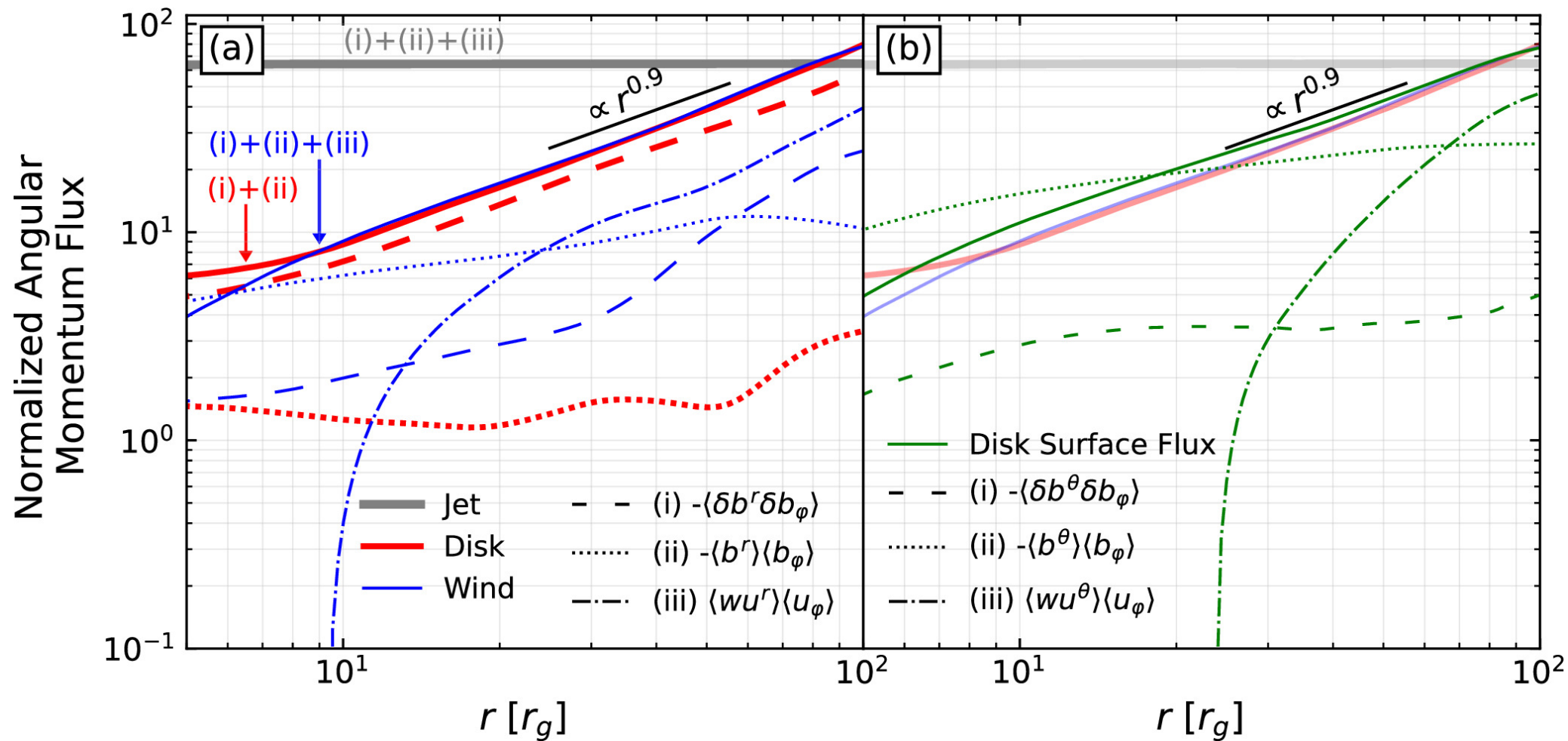
Figure 4. from Vikram Manikantan et al 2024 Astrophys. J. 965 doi:10.3847/1538-4357/ad323d https://dx.doi.org/10.3847/1538-4357/ad323d © 2024. The Author(s). Published by the American Astronomical Society.
