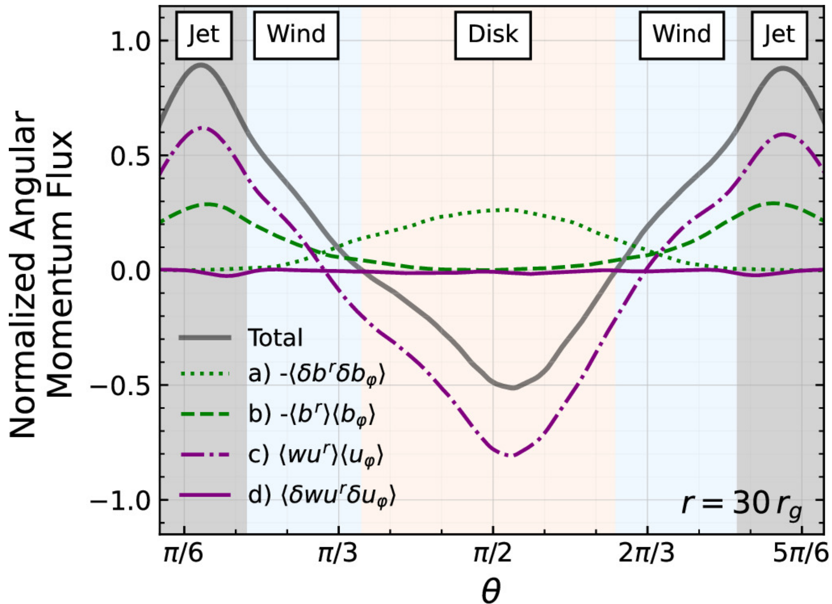
Figure 3. from Vikram Manikantan et al 2024 Astrophys. J. 965 doi:10.3847/1538-4357/ad323d https://dx.doi.org/10.3847/1538-4357/ad323d © 2024. The Author(s). Published by the American Astronomical Society.
