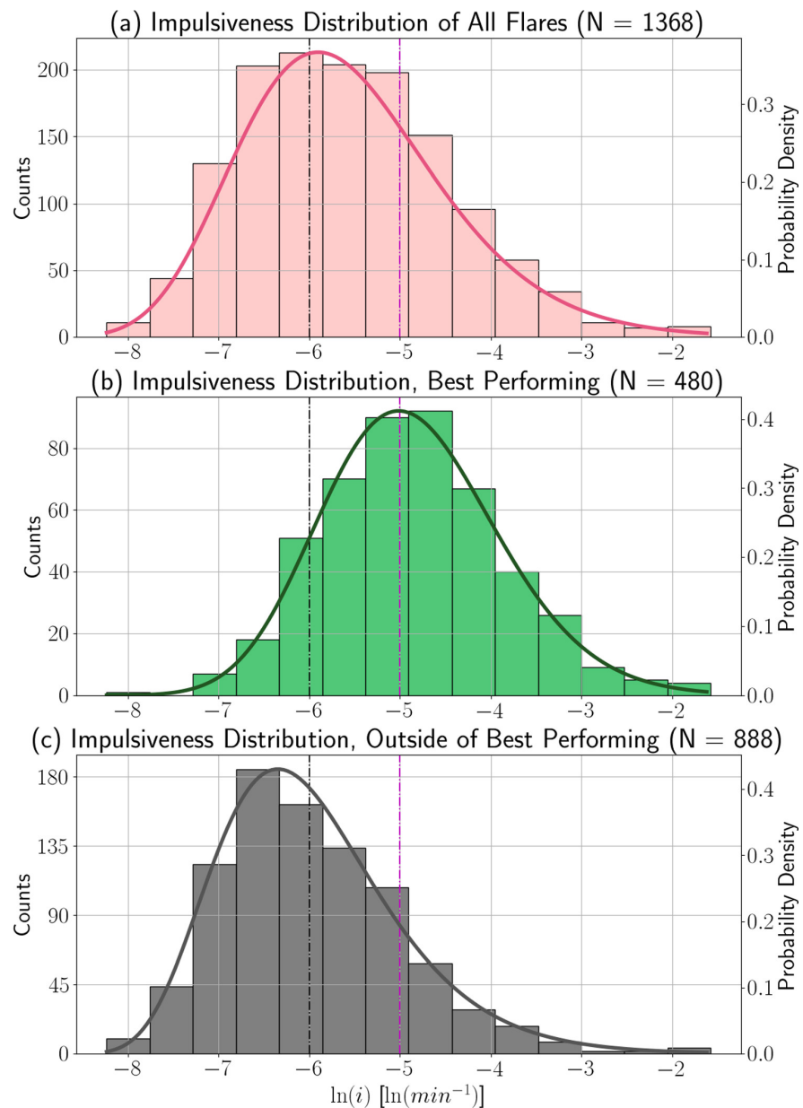
Figure 10. from Cole A. Tamburri et al 2024 Astrophys. J. 966 doi:10.3847/1538-4357/ad3047 https://dx.doi.org/10.3847/1538-4357/ad3047 © 2024. The Author(s). Published by the American Astronomical Society.
