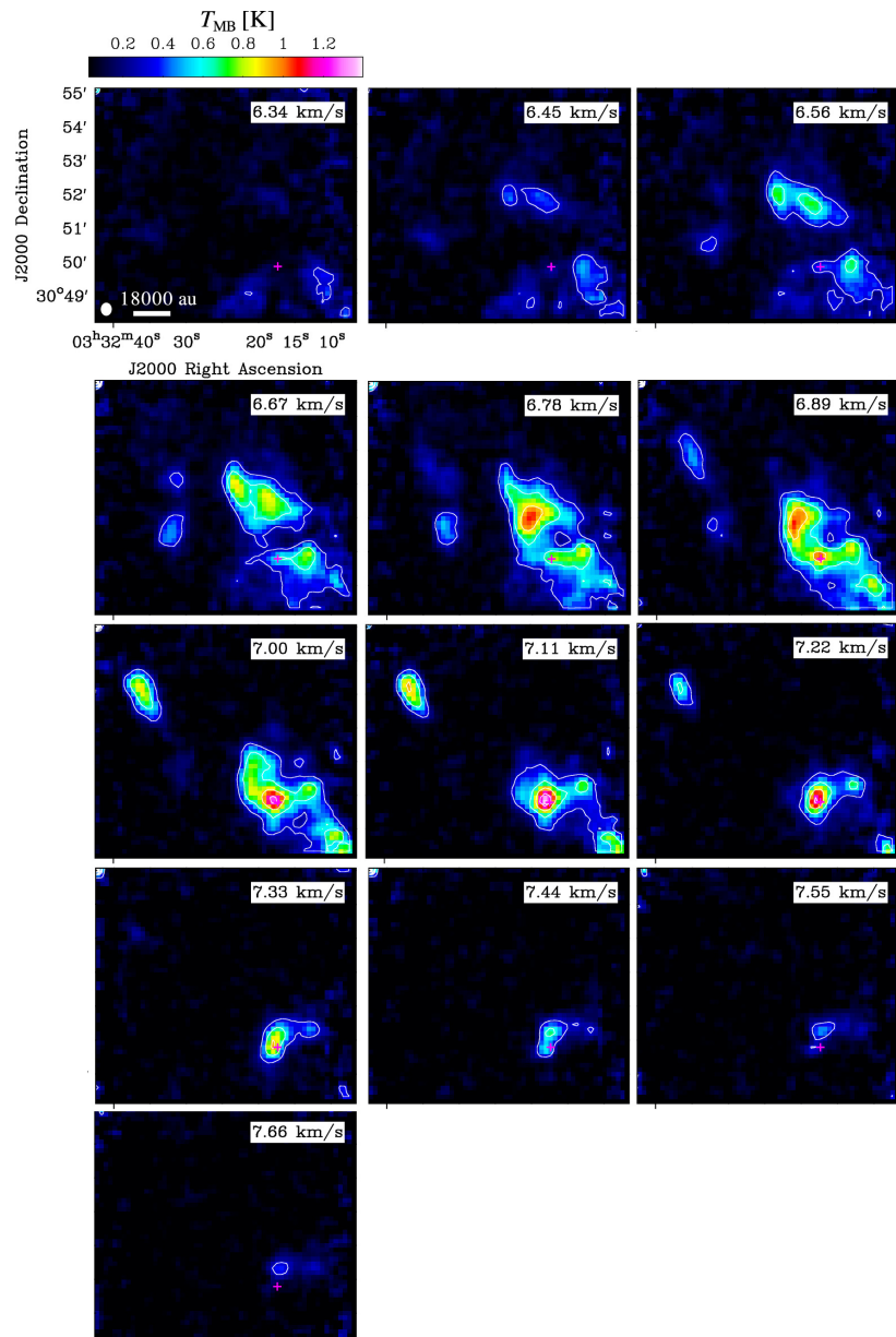
Figure 9. from Kotomi Taniguchi et al 2024 Astrophys. J. 965 doi:10.3847/1538-4357/ad2fa1 https://dx.doi.org/10.3847/1538-4357/ad2fa1 © 2024. The Author(s). Published by the American Astronomical Society.
