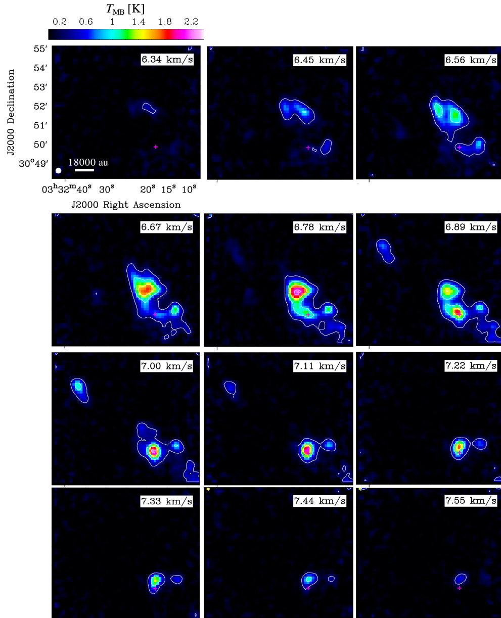
Figure 7. from Kotomi Taniguchi et al 2024 Astrophys. J. 965 doi:10.3847/1538-4357/ad2fa1 https://dx.doi.org/10.3847/1538-4357/ad2fa1 © 2024. The Author(s). Published by the American Astronomical Society.
