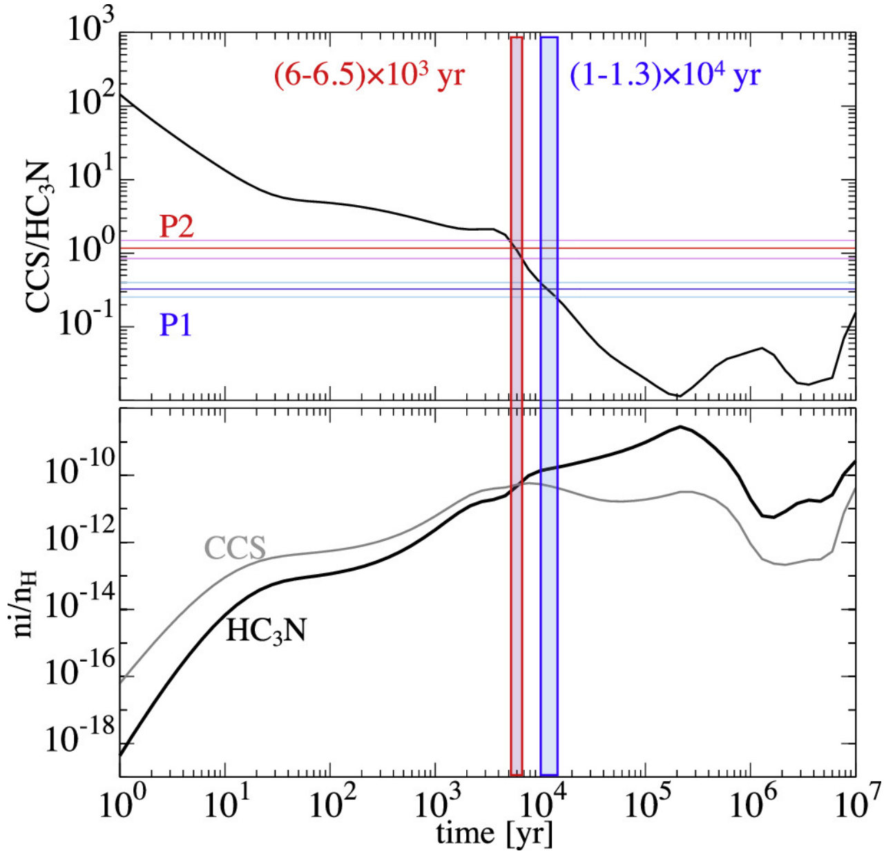
Figure 6. from Kotomi Taniguchi et al 2024 Astrophys. J. 965 doi:10.3847/1538-4357/ad2fa1 https://dx.doi.org/10.3847/1538-4357/ad2fa1 © 2024. The Author(s). Published by the American Astronomical Society.
