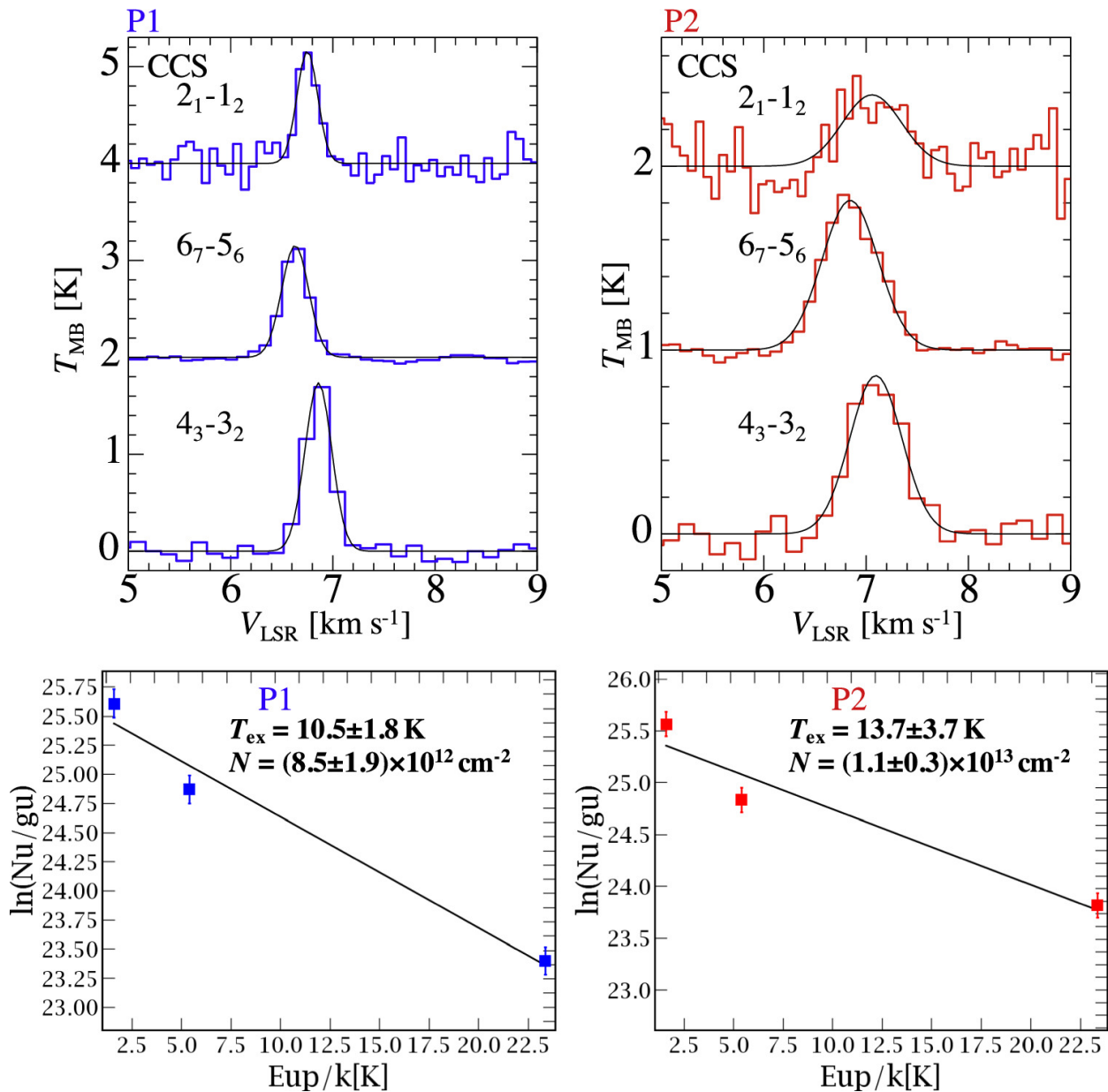
Figure 4. from Kotomi Taniguchi et al 2024 Astrophys. J. 965 doi:10.3847/1538-4357/ad2fa1 https://dx.doi.org/10.3847/1538-4357/ad2fa1 © 2024. The Author(s). Published by the American Astronomical Society.
