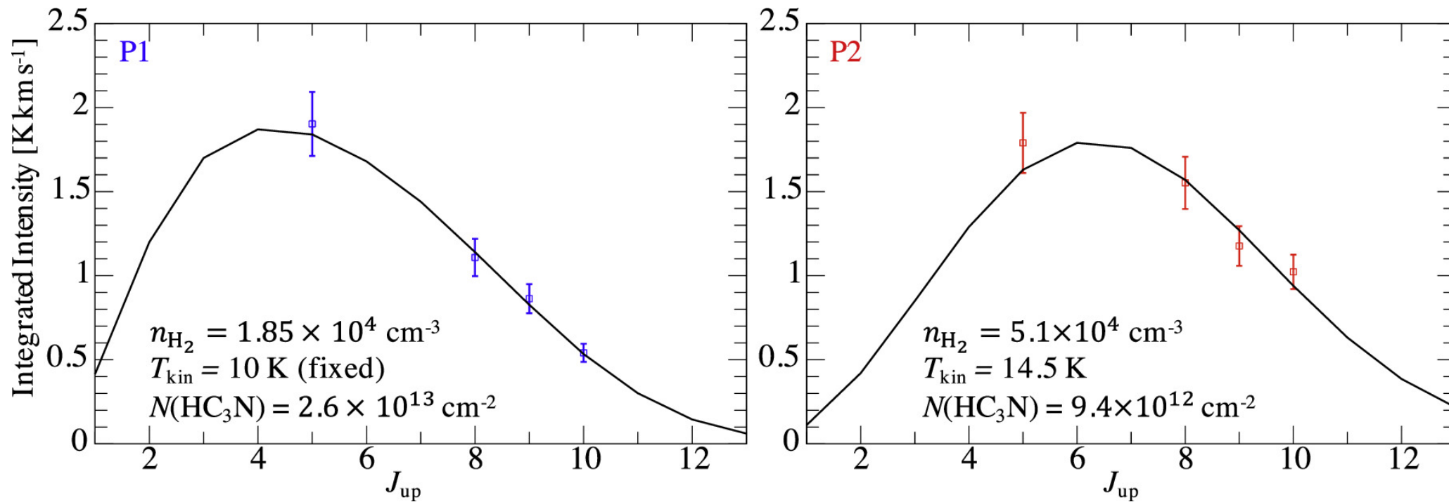
Figure 3. from Kotomi Taniguchi et al 2024 Astrophys. J. 965 doi:10.3847/1538-4357/ad2fa1 https://dx.doi.org/10.3847/1538-4357/ad2fa1 © 2024. The Author(s). Published by the American Astronomical Society.
