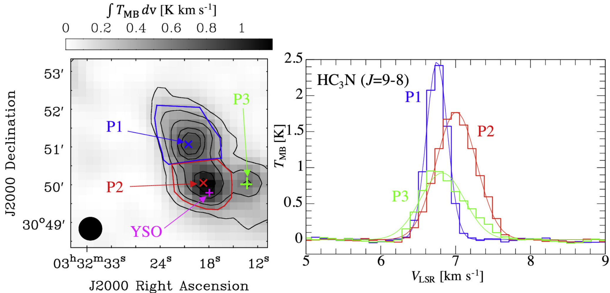
Figure 2. from Kotomi Taniguchi et al 2024 Astrophys. J. 965 doi:10.3847/1538-4357/ad2fa1 https://dx.doi.org/10.3847/1538-4357/ad2fa1 © 2024. The Author(s). Published by the American Astronomical Society.
