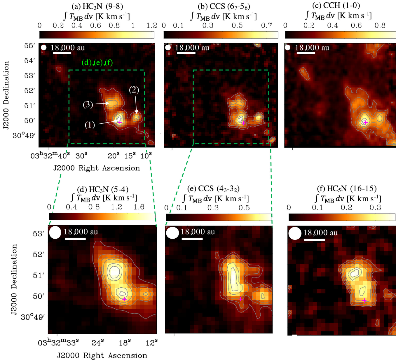
Figure 1. from Kotomi Taniguchi et al 2024 Astrophys. J. 965 doi:10.3847/1538-4357/ad2fa1 https://dx.doi.org/10.3847/1538-4357/ad2fa1 © 2024. The Author(s). Published by the American Astronomical Society.
