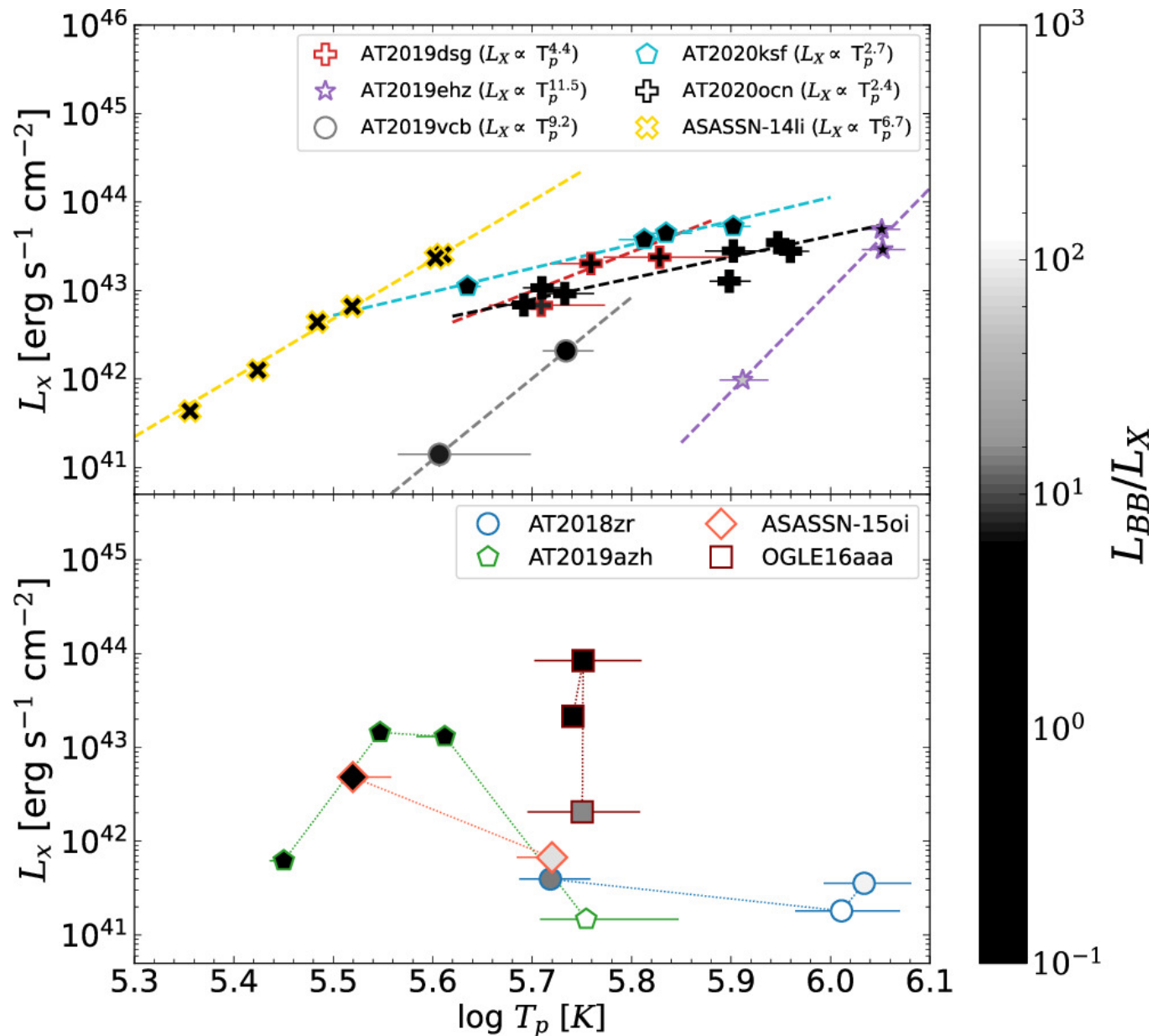
Figure 9. from Muryel Guolo et al 2024 Astrophys. J. 966 doi:10.3847/1538-4357/ad2f9f https://dx.doi.org/10.3847/1538-4357/ad2f9f © 2024. The Author(s). Published by the American Astronomical Society.
