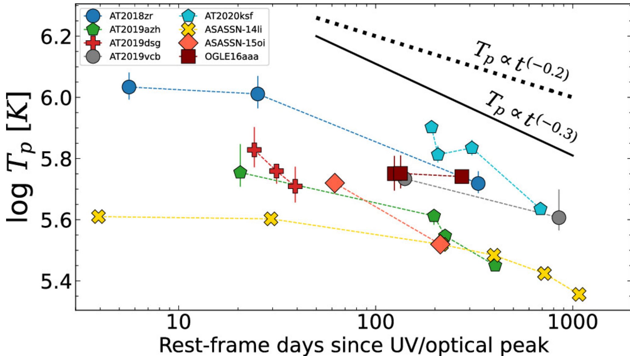
Figure 8. from Muryel Guolo et al 2024 Astrophys. J. 966 doi:10.3847/1538-4357/ad2f9f https://dx.doi.org/10.3847/1538-4357/ad2f9f © 2024. The Author(s). Published by the American Astronomical Society.
