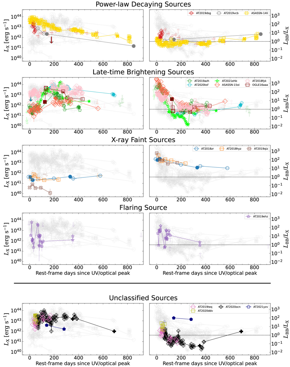
Figure 7. from Muryel Guolo et al 2024 Astrophys. J. 966 doi:10.3847/1538-4357/ad2f9f https://dx.doi.org/10.3847/1538-4357/ad2f9f © 2024. The Author(s). Published by the American Astronomical Society.
