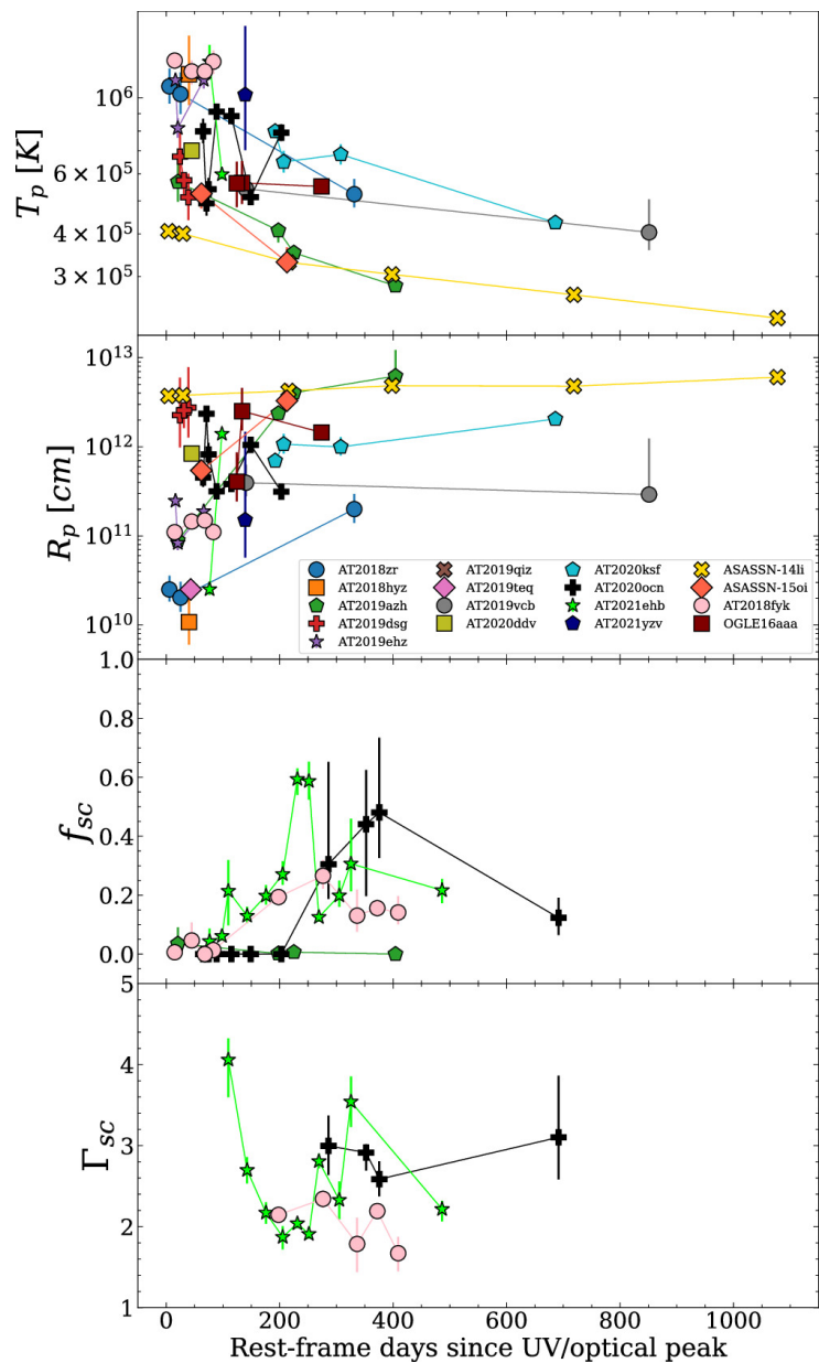
Figure 5. from Muryel Guolo et al 2024 Astrophys. J. 966 doi:10.3847/1538-4357/ad2f9f https://dx.doi.org/10.3847/1538-4357/ad2f9f © 2024. The Author(s). Published by the American Astronomical Society.
