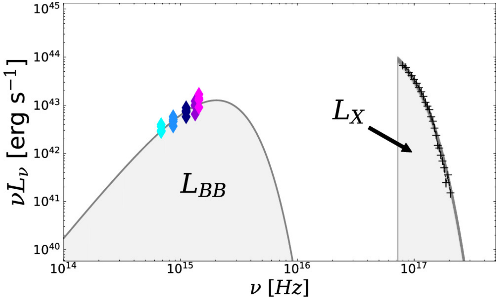
Figure 3. from Muryel Guolo et al 2024 Astrophys. J. 966 doi:10.3847/1538-4357/ad2f9f https://dx.doi.org/10.3847/1538-4357/ad2f9f © 2024. The Author(s). Published by the American Astronomical Society.
