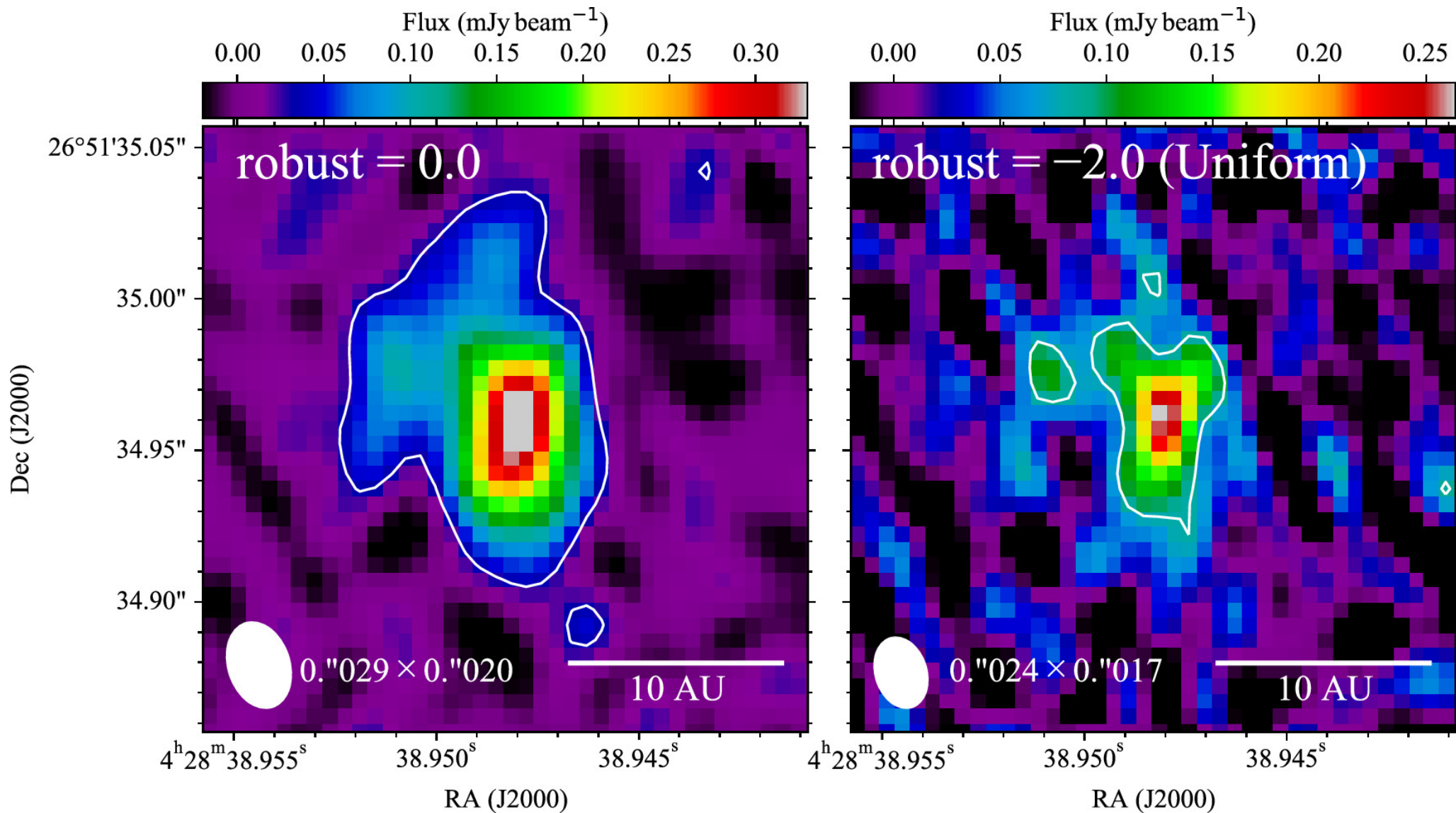
Figure A1. from Kazuki Tokuda et al 2024 Astrophys. J. 965 doi:10.3847/1538-4357/ad2f9a https://dx.doi.org/10.3847/1538-4357/ad2f9a © 2024. The Author(s). Published by the American Astronomical Society.
