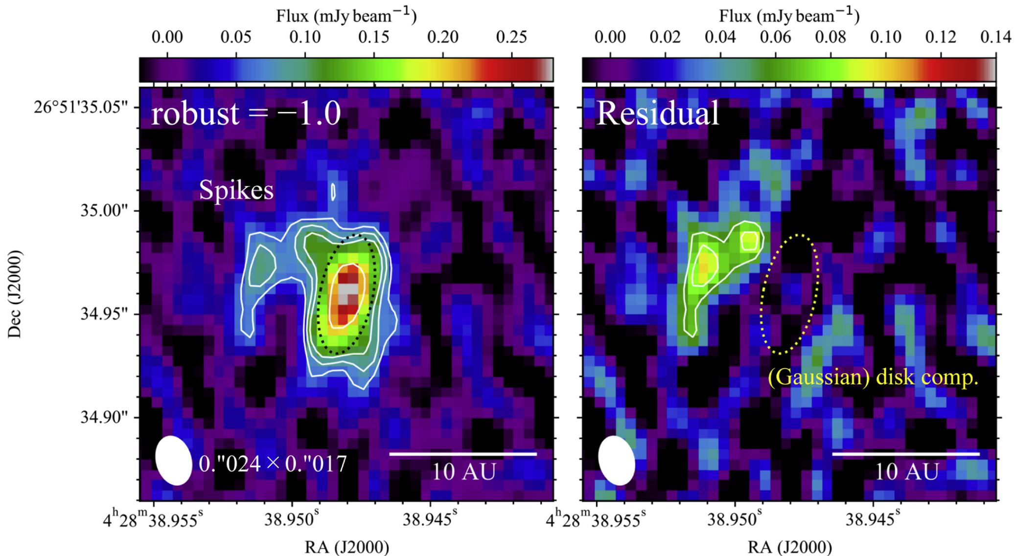
Figure 1. from Kazuki Tokuda et al 2024 Astrophys. J. 965 doi:10.3847/1538-4357/ad2f9a https://dx.doi.org/10.3847/1538-4357/ad2f9a © 2024. The Author(s). Published by the American Astronomical Society.
