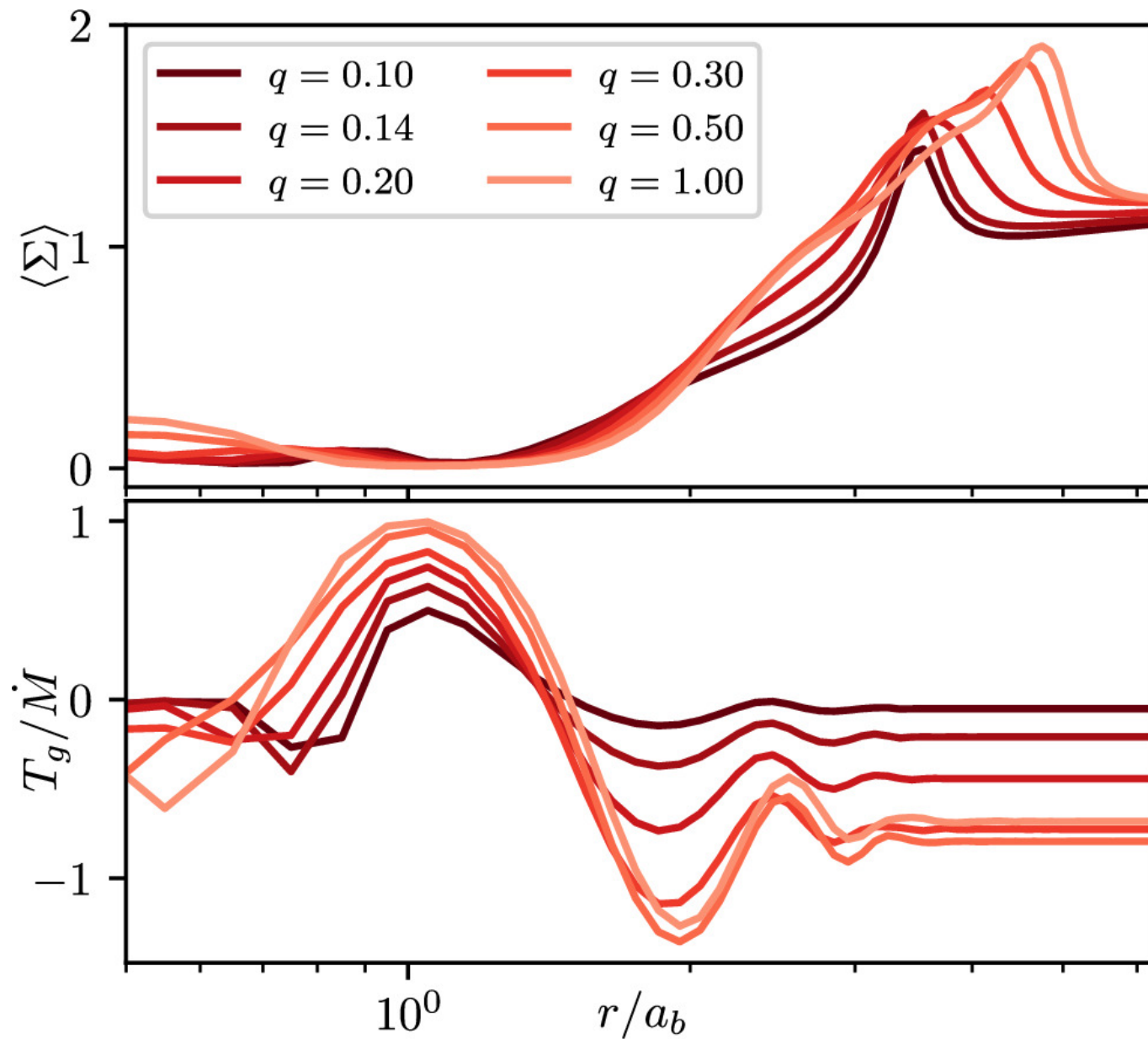
Figure 8. from Alexander J. Dittmann and Geoffrey Ryan 2024 Astrophys. J. 967 doi:10.3847/1538-4357/ad2f1e https://dx.doi.org/10.3847/1538-4357/ad2f1e © 2024. The Author(s). Published by the American Astronomical Society.
