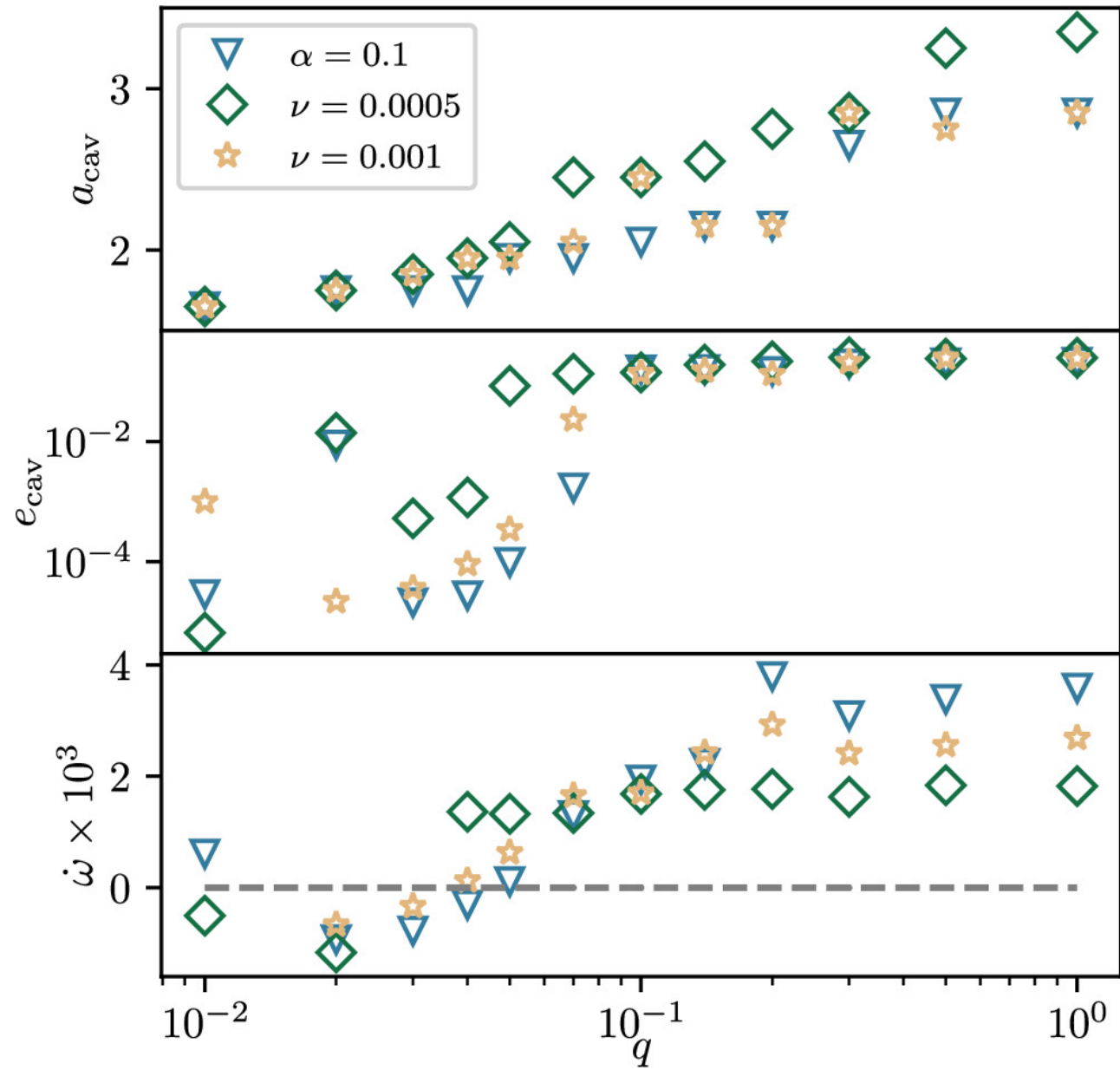
Figure 7. from Alexander J. Dittmann and Geoffrey Ryan 2024 Astrophys. J. 967 doi:10.3847/1538-4357/ad2f1e https://dx.doi.org/10.3847/1538-4357/ad2f1e © 2024. The Author(s). Published by the American Astronomical Society.
