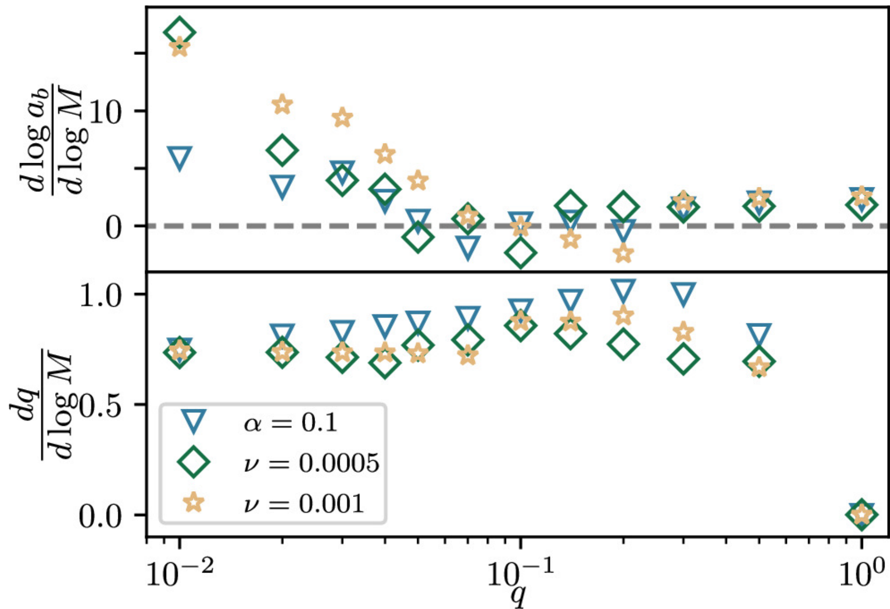
Figure 5. from Alexander J. Dittmann and Geoffrey Ryan 2024 Astrophys. J. 967 doi:10.3847/1538-4357/ad2f1e https://dx.doi.org/10.3847/1538-4357/ad2f1e © 2024. The Author(s). Published by the American Astronomical Society.
