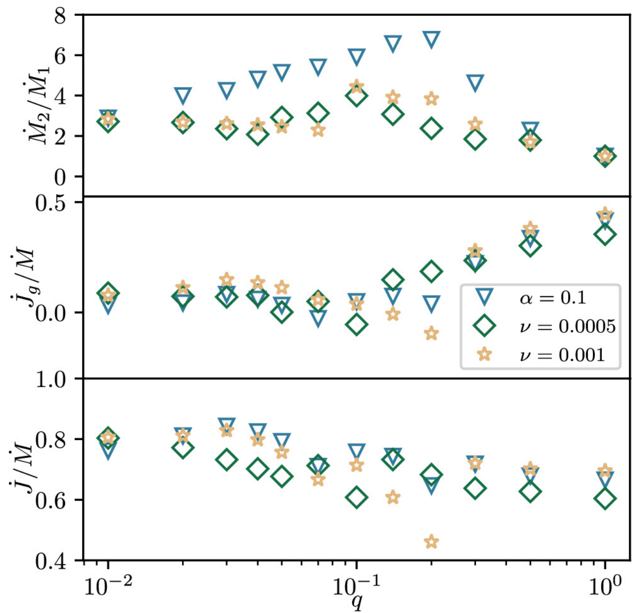
Figure 4. from Alexander J. Dittmann and Geoffrey Ryan 2024 Astrophys. J. 967 doi:10.3847/1538-4357/ad2f1e https://dx.doi.org/10.3847/1538-4357/ad2f1e © 2024. The Author(s). Published by the American Astronomical Society.
