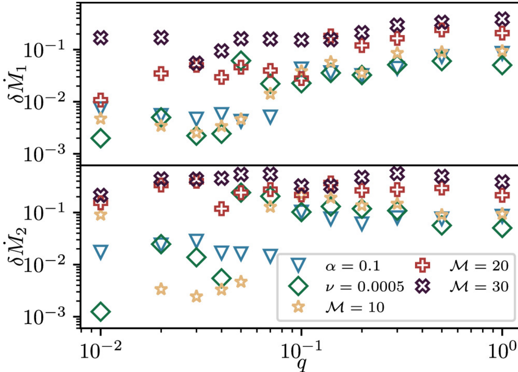
Figure 15. from Alexander J. Dittmann and Geoffrey Ryan 2024 Astrophys. J. 967 doi:10.3847/1538-4357/ad2f1e https://dx.doi.org/10.3847/1538-4357/ad2f1e © 2024. The Author(s). Published by the American Astronomical Society.
