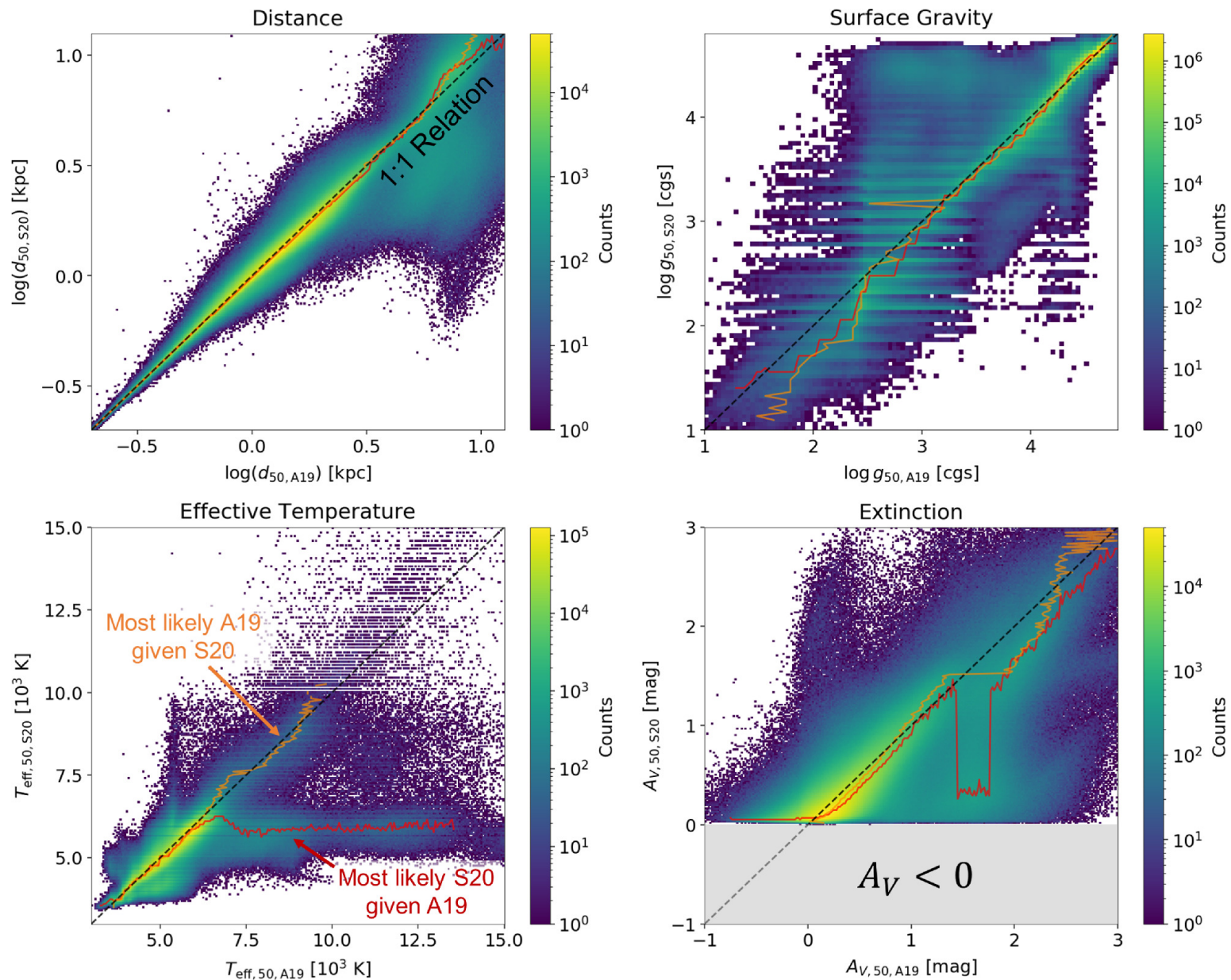
Figure 9. from Joshua S. Speagle et al 2024 Astrophys. J. 970 doi:10.3847/1538-4357/ad2b62 https://dx.doi.org/10.3847/1538-4357/ad2b62 © 2024. The Author(s). Published by the American Astronomical Society.
