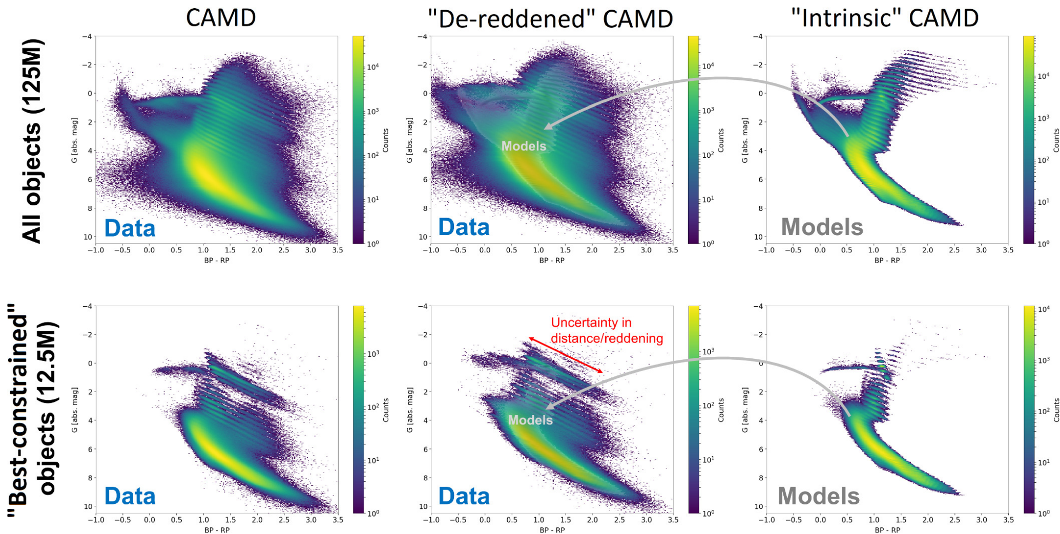
Figure 8. from Joshua S. Speagle et al 2024 Astrophys. J. 970 doi:10.3847/1538-4357/ad2b62 https://dx.doi.org/10.3847/1538-4357/ad2b62 © 2024. The Author(s). Published by the American Astronomical Society.
