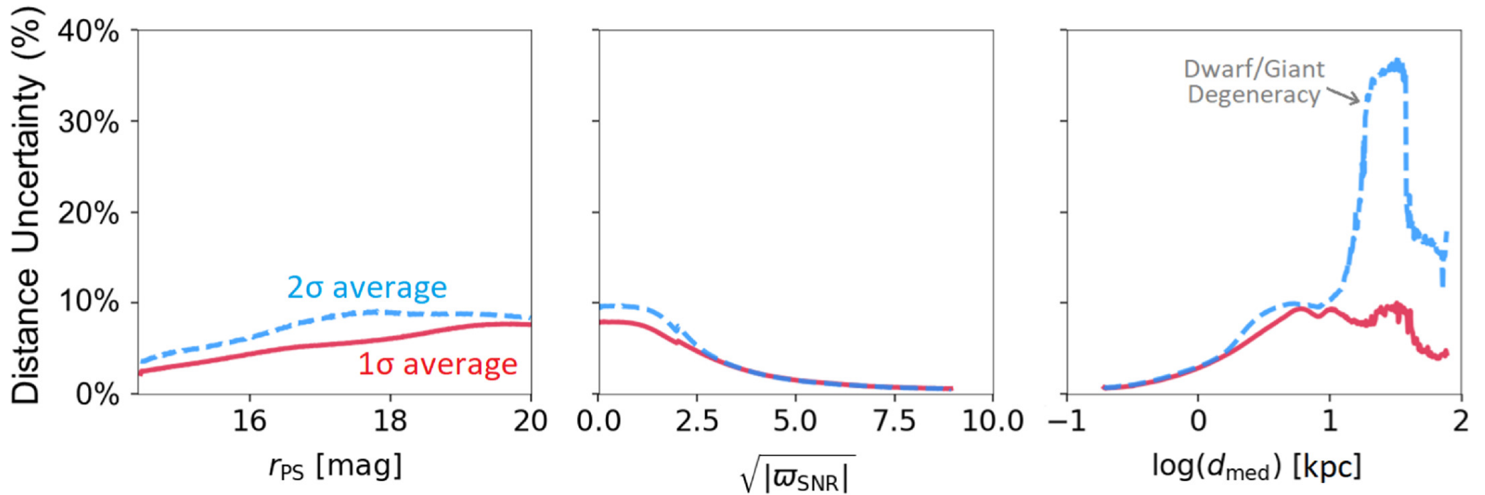
Figure 6. from Joshua S. Speagle et al 2024 Astrophys. J. 970 doi:10.3847/1538-4357/ad2b62 https://dx.doi.org/10.3847/1538-4357/ad2b62 © 2024. The Author(s). Published by the American Astronomical Society.
