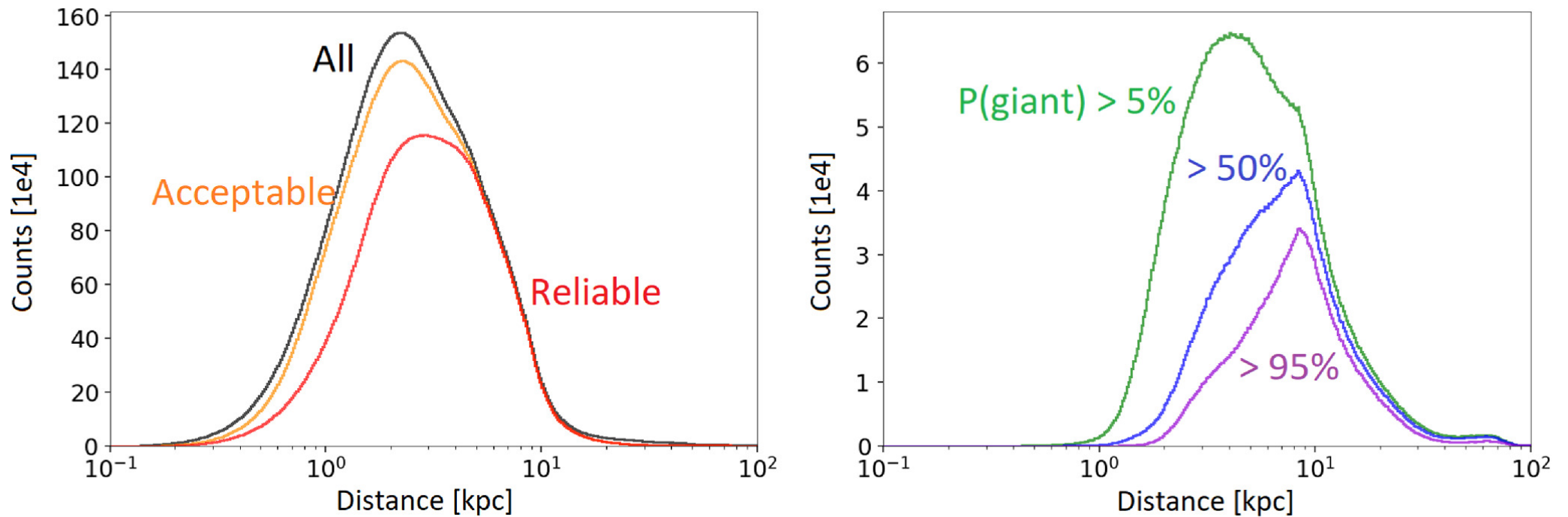
Figure 5. from Joshua S. Speagle et al 2024 Astrophys. J. 970 doi:10.3847/1538-4357/ad2b62 https://dx.doi.org/10.3847/1538-4357/ad2b62 © 2024. The Author(s). Published by the American Astronomical Society.
