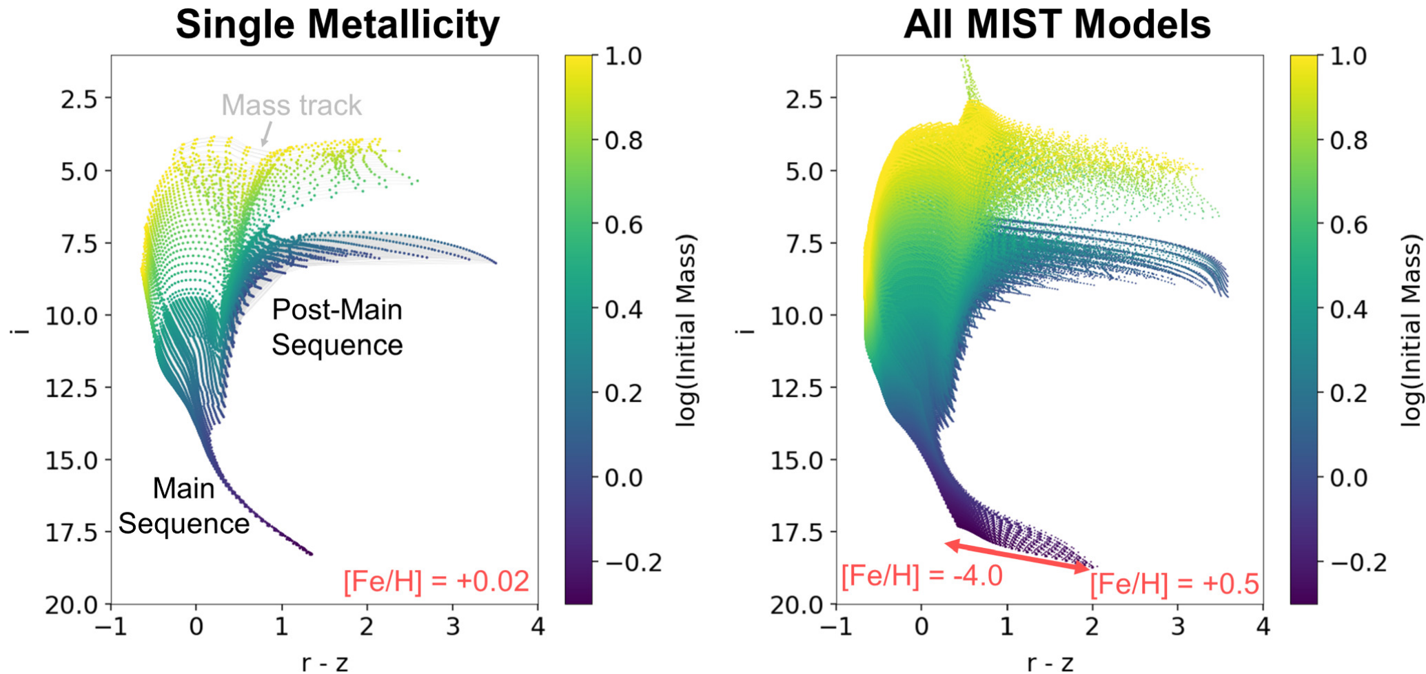
Figure 4. from Joshua S. Speagle et al 2024 Astrophys. J. 970 doi:10.3847/1538-4357/ad2b62 https://dx.doi.org/10.3847/1538-4357/ad2b62 © 2024. The Author(s). Published by the American Astronomical Society.
