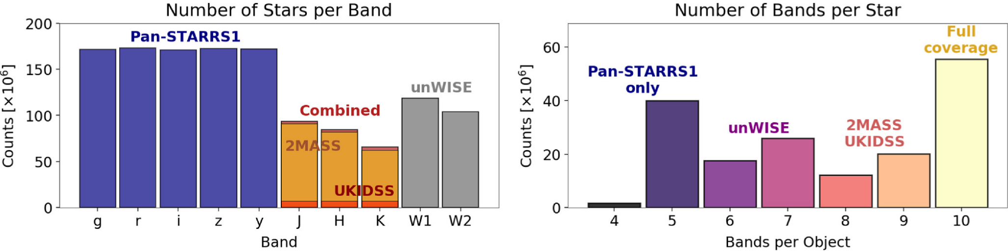
Figure 3. from Joshua S. Speagle et al 2024 Astrophys. J. 970 doi:10.3847/1538-4357/ad2b62 https://dx.doi.org/10.3847/1538-4357/ad2b62 © 2024. The Author(s). Published by the American Astronomical Society.
