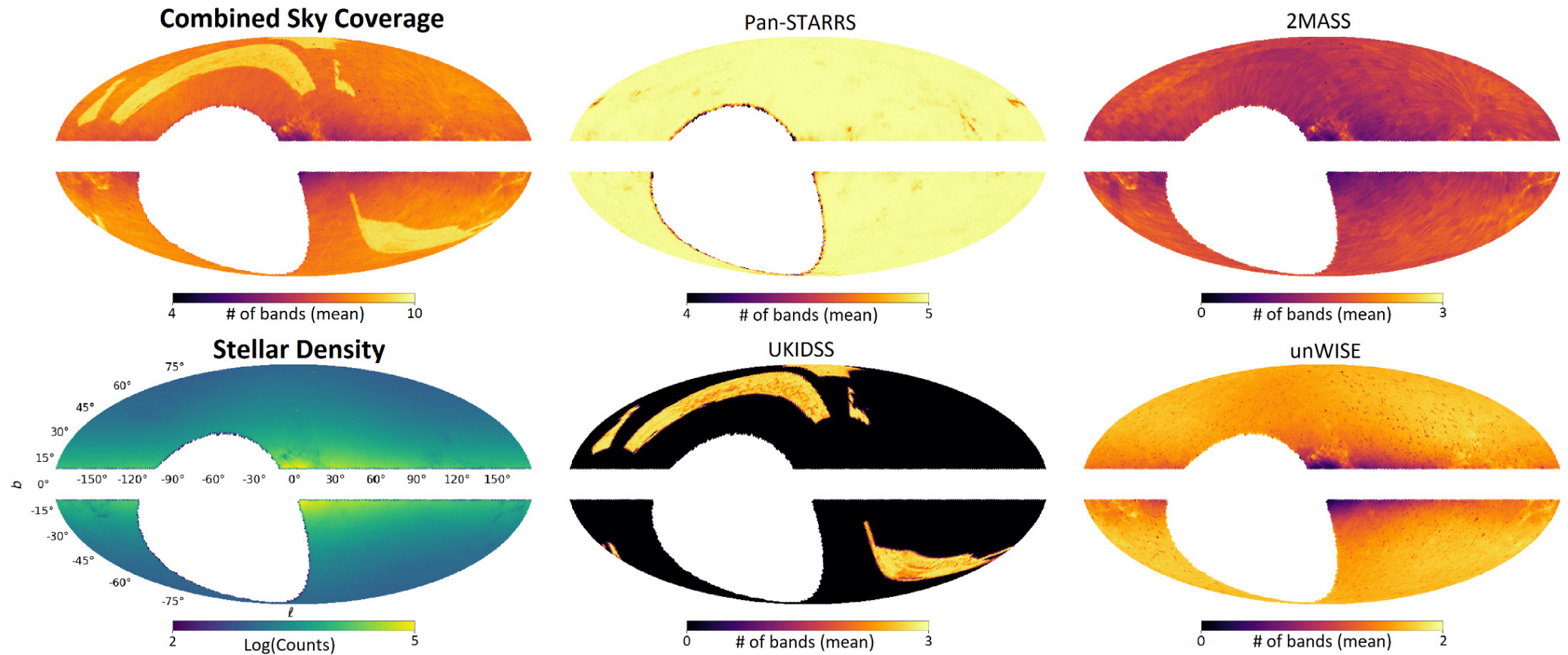
Figure 2. from Joshua S. Speagle et al 2024 Astrophys. J. 970 doi:10.3847/1538-4357/ad2b62 https://dx.doi.org/10.3847/1538-4357/ad2b62 © 2024. The Author(s). Published by the American Astronomical Society.
