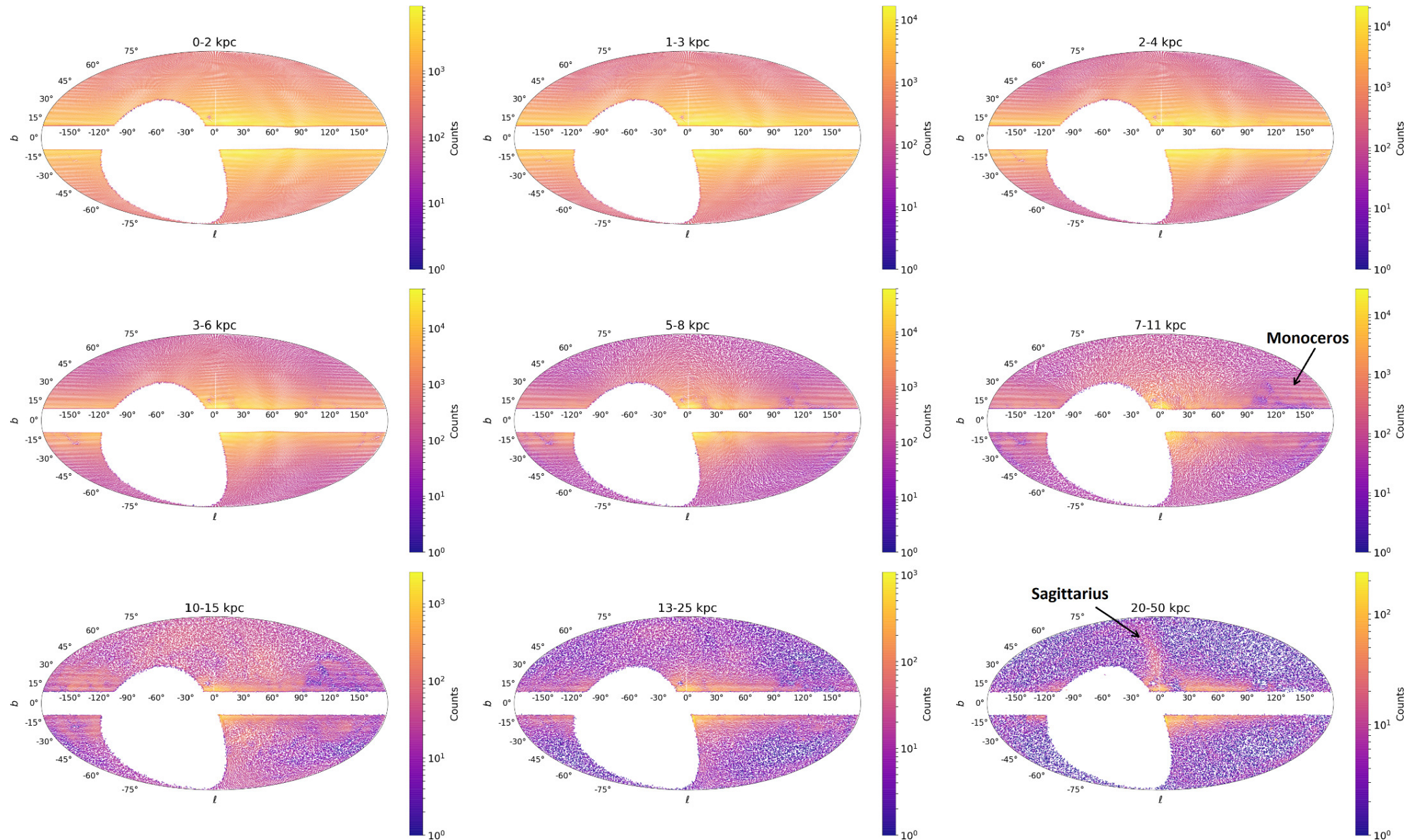
Figure 11. from Joshua S. Speagle et al 2024 Astrophys. J. 970 doi:10.3847/1538-4357/ad2b62 https://dx.doi.org/10.3847/1538-4357/ad2b62 © 2024. The Author(s). Published by the American Astronomical Society.
