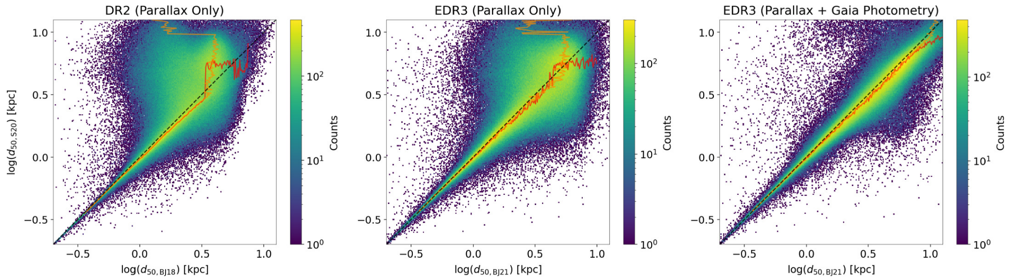
Figure 10. from Joshua S. Speagle et al 2024 Astrophys. J. 970 doi:10.3847/1538-4357/ad2b62 https://dx.doi.org/10.3847/1538-4357/ad2b62 © 2024. The Author(s). Published by the American Astronomical Society.
