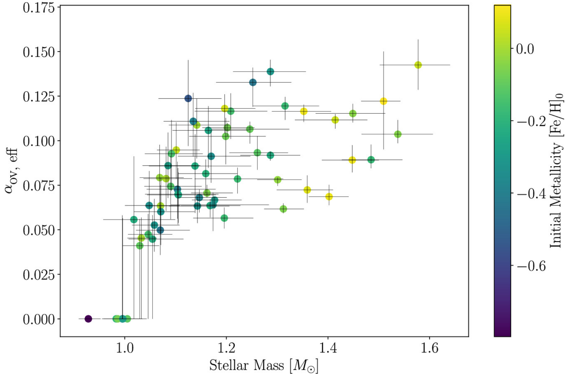
Figure 6. from Christopher J. Lindsay et al 2024 Astrophys. J. 965 doi:10.3847/1538-4357/ad2ae5 https://dx.doi.org/10.3847/1538-4357/ad2ae5 © 2024. The Author(s). Published by the American Astronomical Society.
