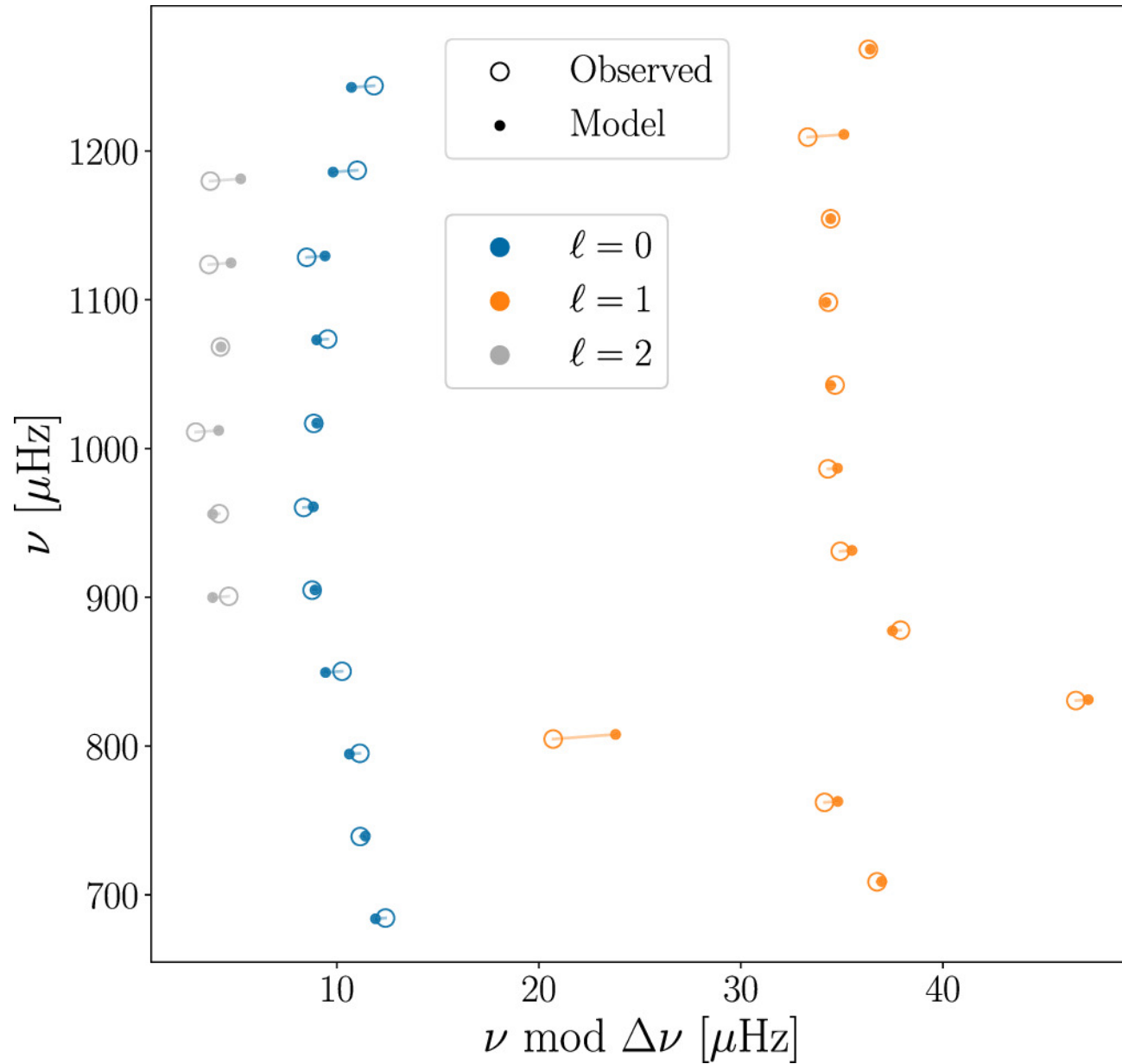
Figure 5. from Christopher J. Lindsay et al 2024 Astrophys. J. 965 doi:10.3847/1538-4357/ad2ae5 https://dx.doi.org/10.3847/1538-4357/ad2ae5 © 2024. The Author(s). Published by the American Astronomical Society.
