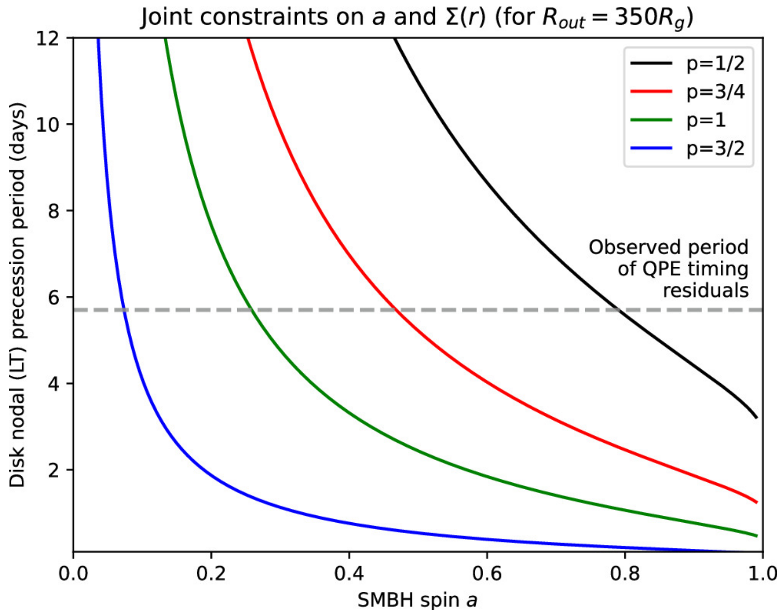
Figure 8. from Joheen Chakraborty et al 2024 Astrophys. J. 965 doi:10.3847/1538-4357/ad2941 https://dx.doi.org/10.3847/1538-4357/ad2941 © 2024. The Author(s). Published by the American Astronomical Society.
