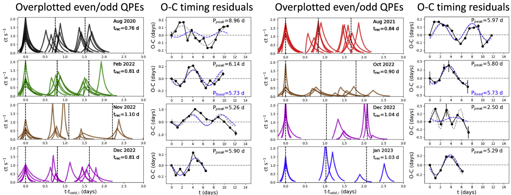
Figure 7. from Joheen Chakraborty et al 2024 Astrophys. J. 965 doi:10.3847/1538-4357/ad2941 https://dx.doi.org/10.3847/1538-4357/ad2941
