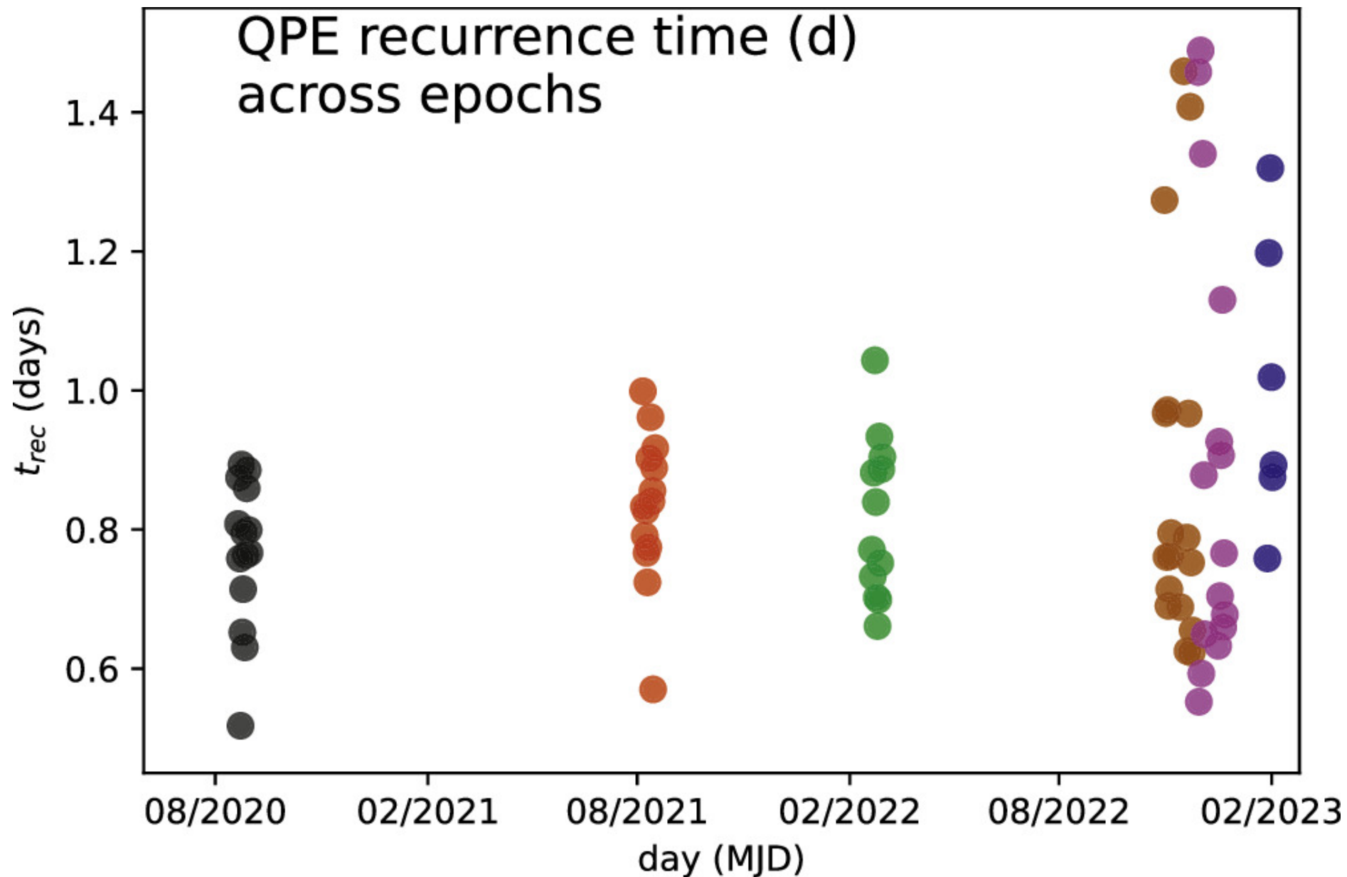
Figure 6. from Joheen Chakraborty et al 2024 Astrophys. J. 965 doi:10.3847/1538-4357/ad2941 https://dx.doi.org/10.3847/1538-4357/ad2941 © 2024. The Author(s). Published by the American Astronomical Society.
