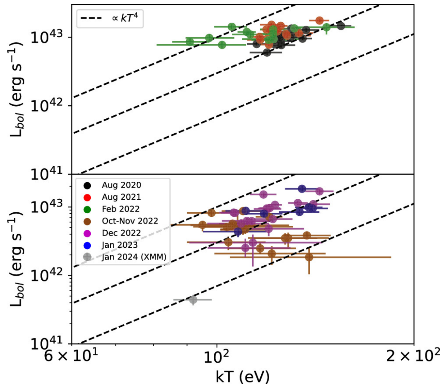
Figure 4. from Joheen Chakraborty et al 2024 Astrophys. J. 965 doi:10.3847/1538-4357/ad2941 https://dx.doi.org/10.3847/1538-4357/ad2941 © 2024. The Author(s). Published by the American Astronomical Society.
