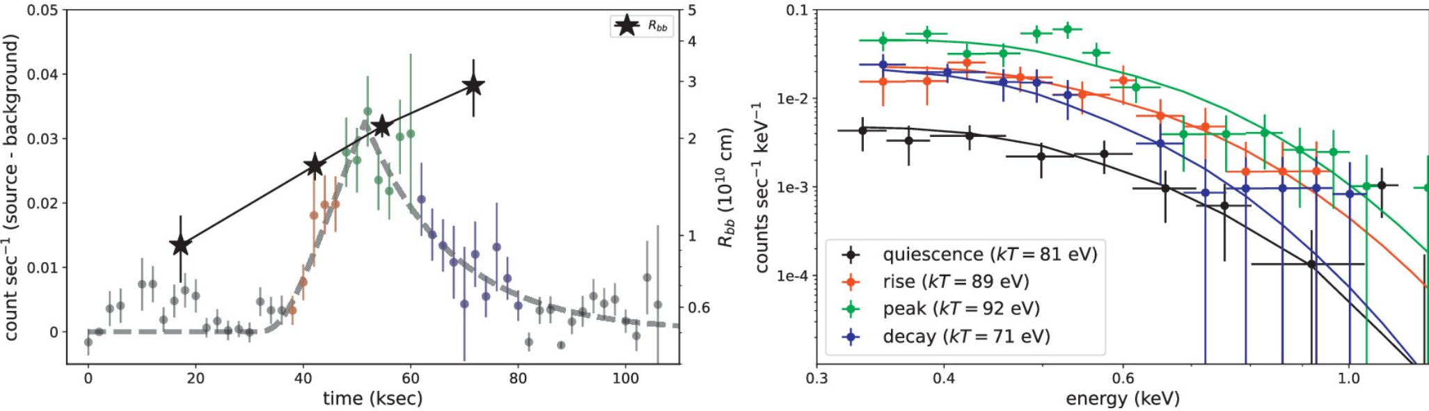
Figure 2. from Joheen Chakraborty et al 2024 Astrophys. J. 965 doi:10.3847/1538-4357/ad2941 https://dx.doi.org/10.3847/1538-4357/ad2941 © 2024. The Author(s). Published by the American Astronomical Society.
